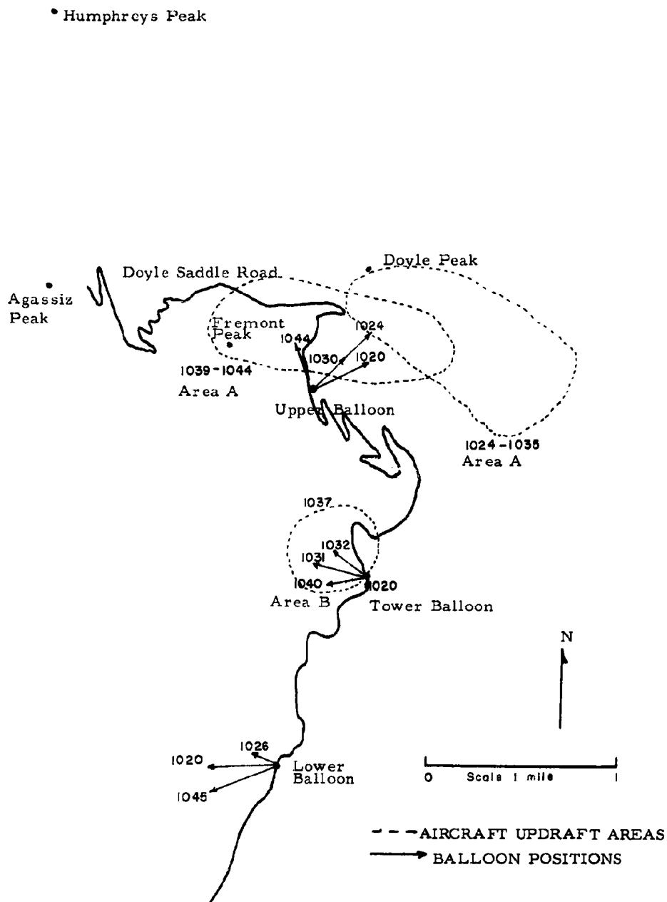
Fig. I-2. CONVECTIVE SLOPE FLOWS (1020 - 1045 MST) JULY 28, 1962
