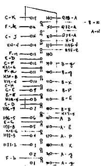
J2 DDM-50S
