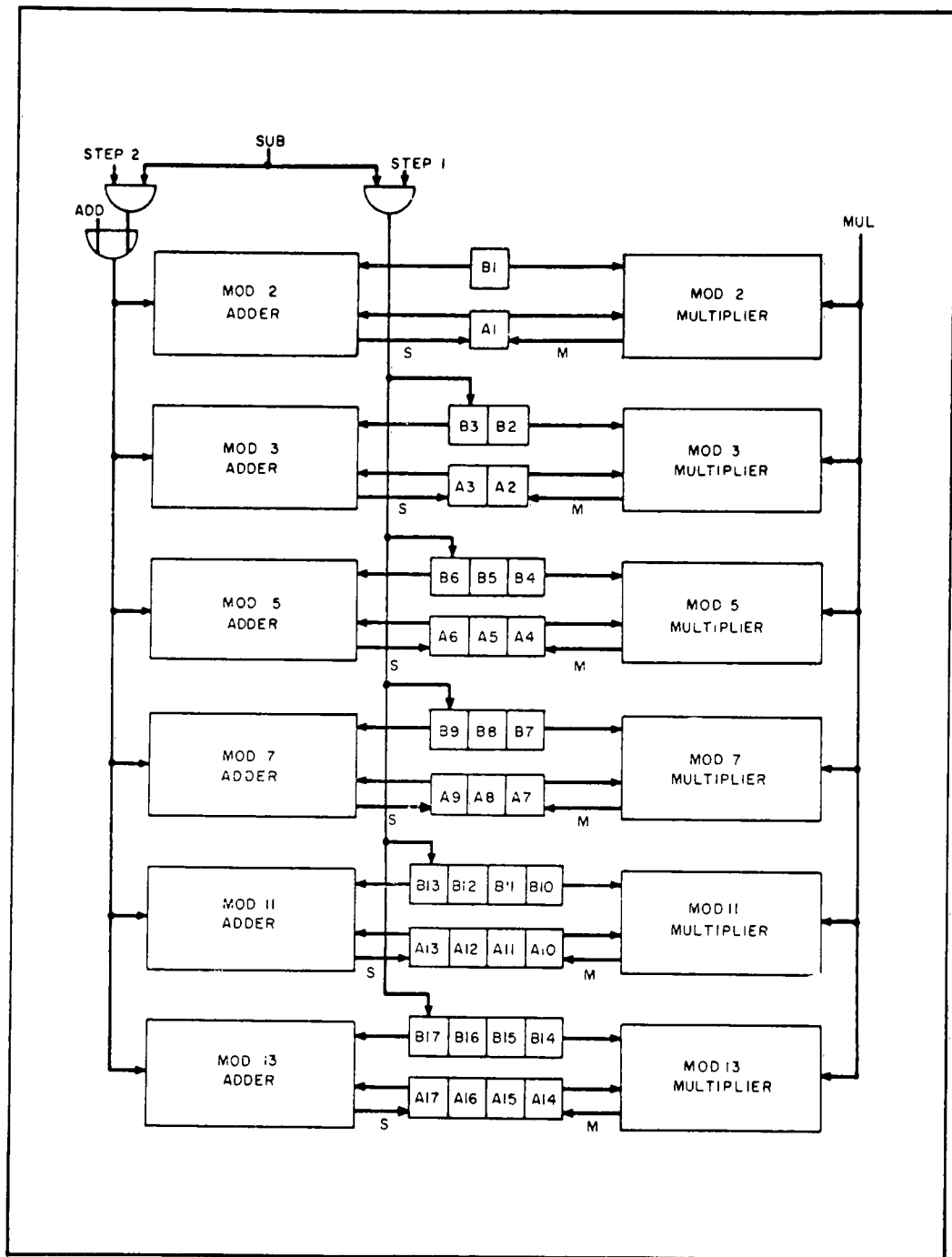
Figure 6-2. Arithmetic Control
