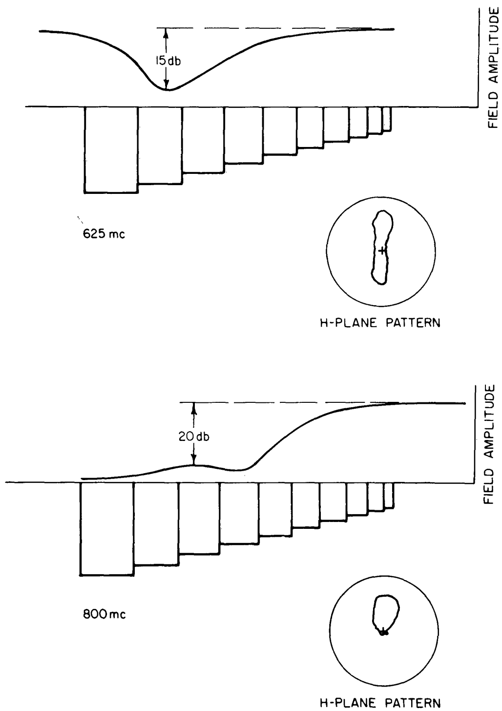
Figure 2.4. Near Field Plots for 625 Mc and 800 Mc
