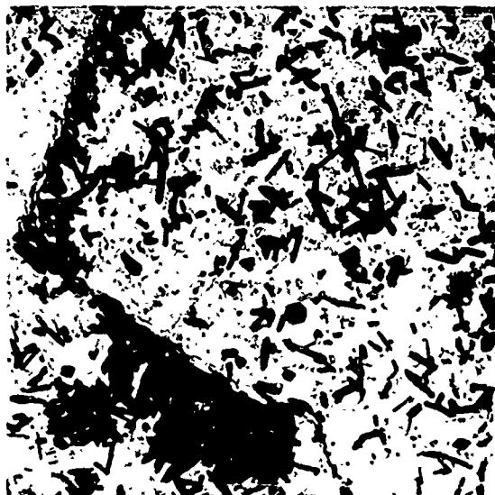
FIGURE 38 - EXTRACTION REPLICA OF Cb-5Hf-0.2N ALLOY, AGED 1 HOUR AT 1600 °C. 5500X
