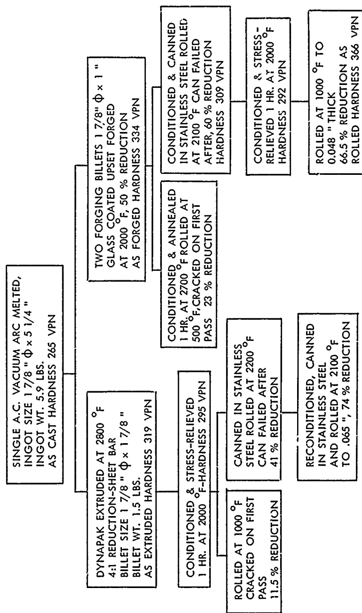
FIGURE 5 - PROCESSING OF B-77 + .075C, HEAT VAM 61
