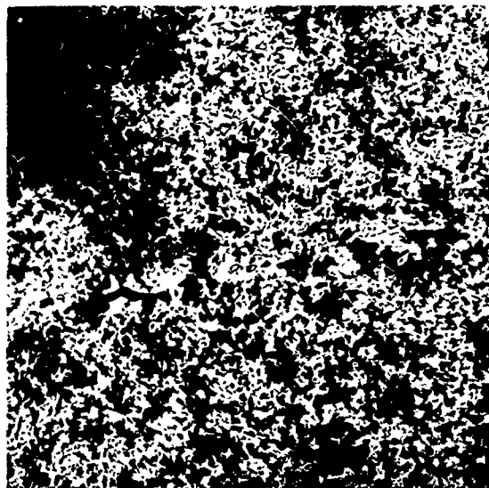
FIGURE 37 - EXTRACTION REPLICA OF Cb-5Hf-0.2N ALLOY, AGED 1 HOUR AT 1400 °C. 5500X
