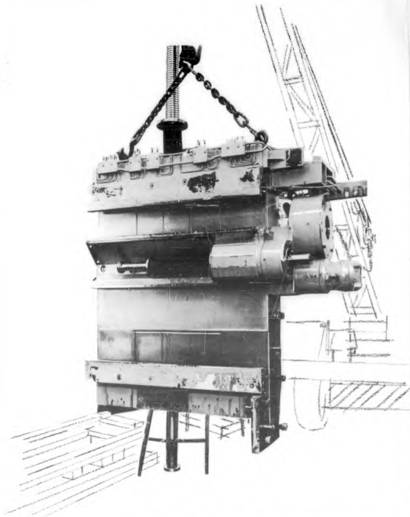
10 FRONT OF SADDLE WITH BALL SCREW ASSEMBLY
