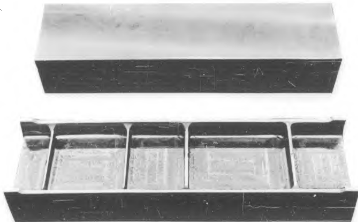
1 PART NO. 263-315217-5 BEFORE AND AFTER MACHINING
