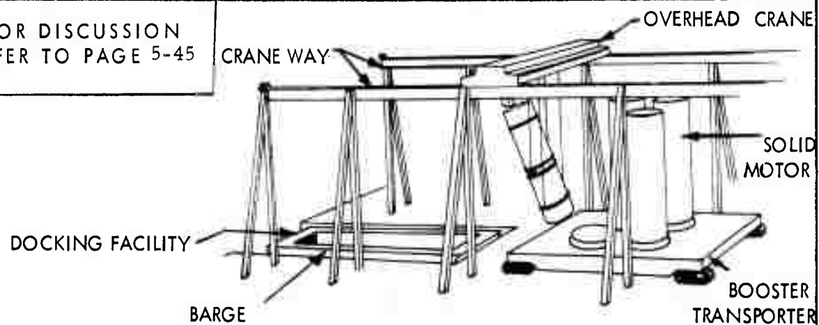
FIGURE 5-40 BOOSTER ASSEMBLY ON MOVABLE TRANSPORTER
