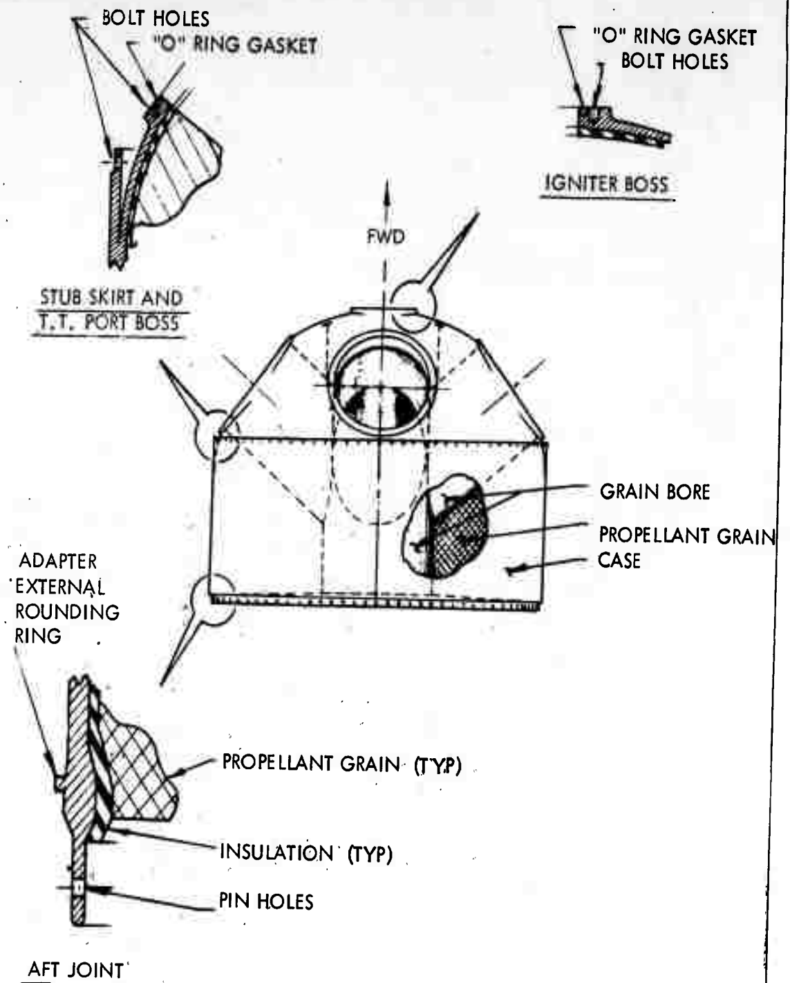
FIGURE 6-6 FORWARD CLOSURE
