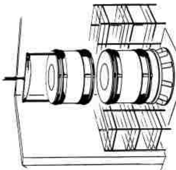
Positioning of Large Solid Marine Segments
