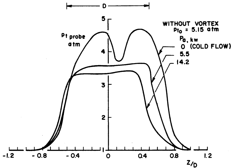
c. Profiles at a Chamber Pressure of 5.15 atm and Several Power Levels
