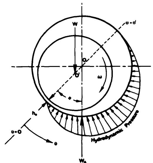
Fig. 27 - Attitude Relationships for Journal Bearing.
