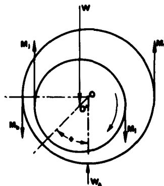
Fig. 23 - Relationship Between Bearing Friction Torque and Journal Friction Torque (9).
