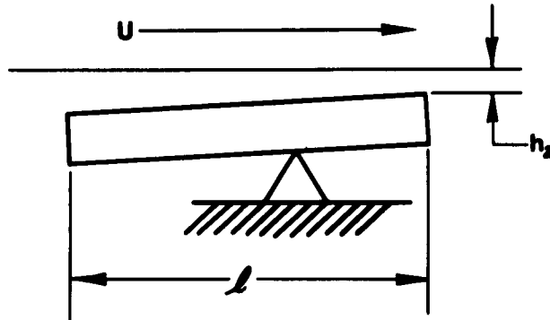
Fig. 4 - Schematic Diagram of Slider Thrust Bearing.
