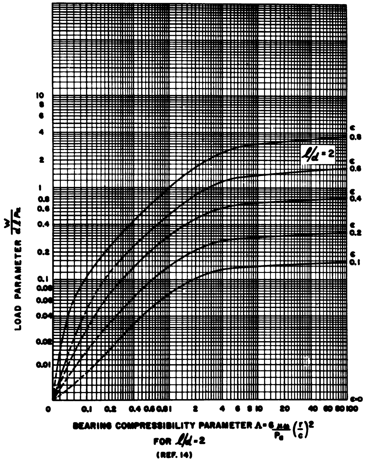
Fig. 13 - Theoretical Load-Carrying Parameter vs Compressibility Parameter for Full Journal Bearing for l/d=2 (Ref. 14)
