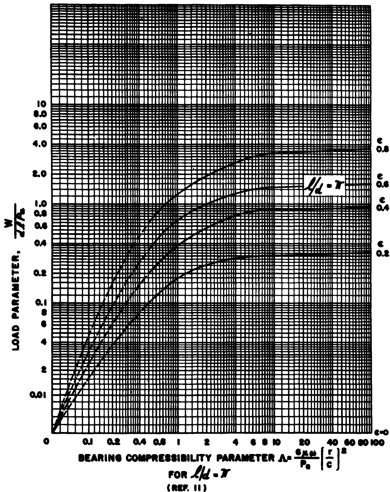
Fig. 12 - Theoretical Load-Carrying Parameter vs Compressibility Parameter for Full Journal Bearing for l/d = \pi (Ref. 11).
