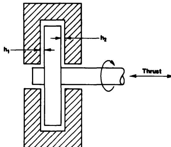
Fig. 62 - Schematic Diagram of Double Acting Thrust Bearing.
