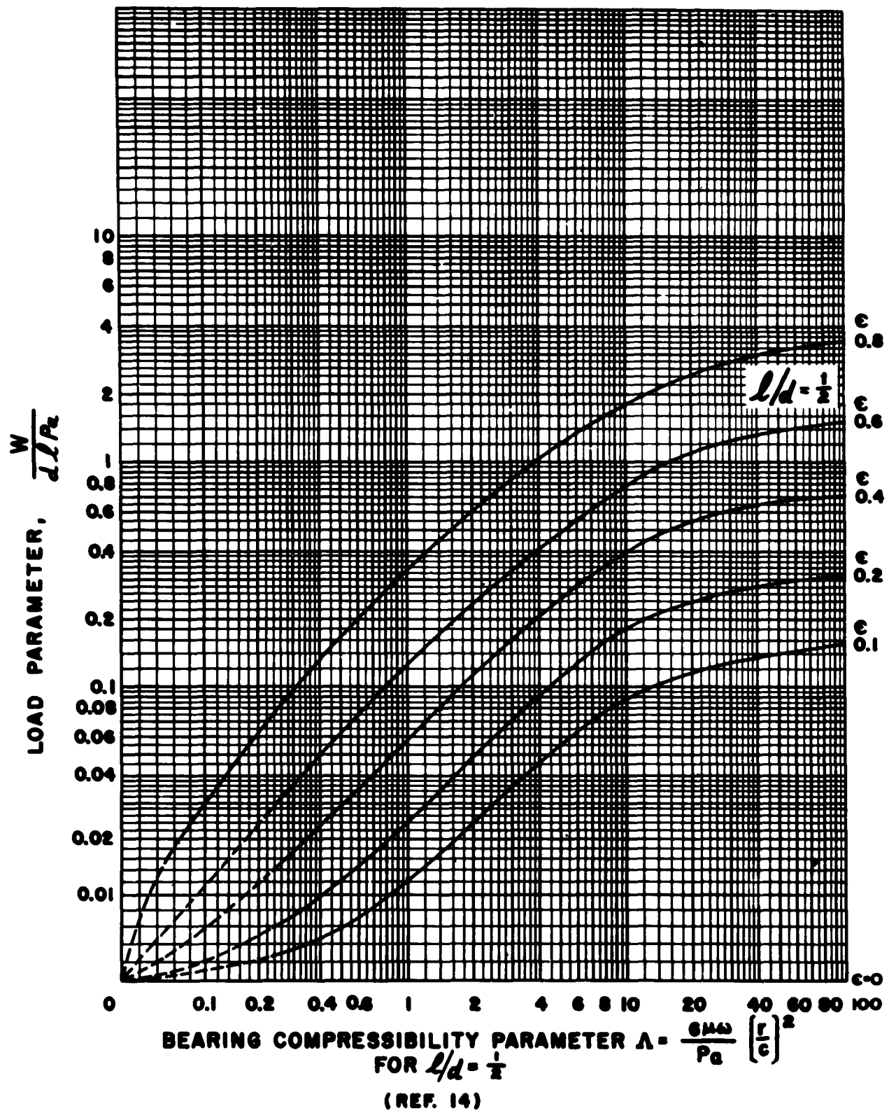
Fig. 15 - Theoretical Load-Carrying Parameter vs Compressibility Parameter for Full Journal Bearing for l/d = \frac{1}{2} (Ref. 14)
