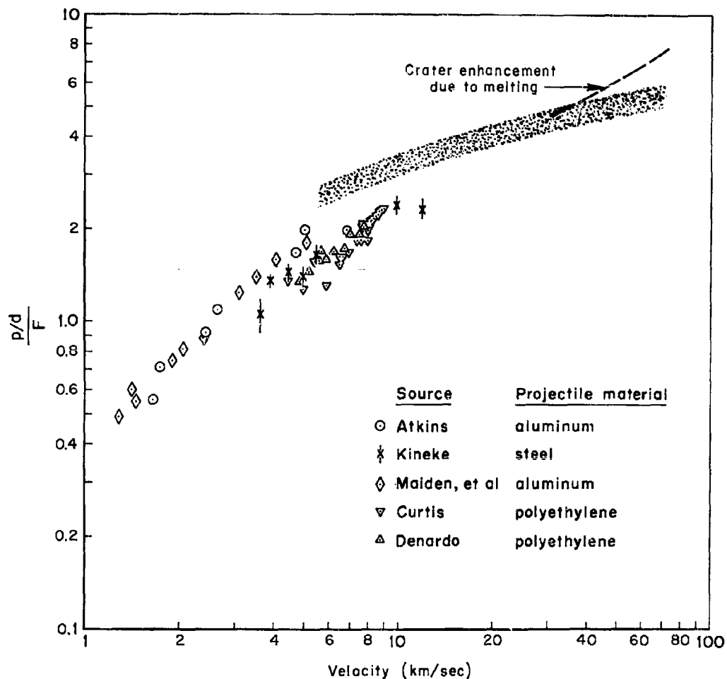
Fig. 19 — Dissimilar-material scaling law compared with experimental data for 2024-T3 targets.
