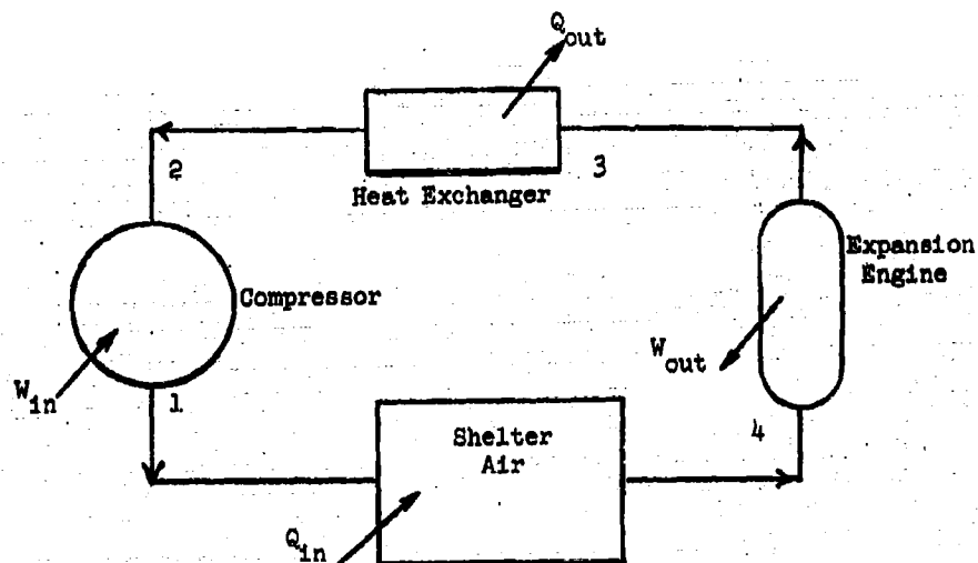
Figure 20 FLOW DIAGRAM FOR AIR CYCLE SYSTEM
