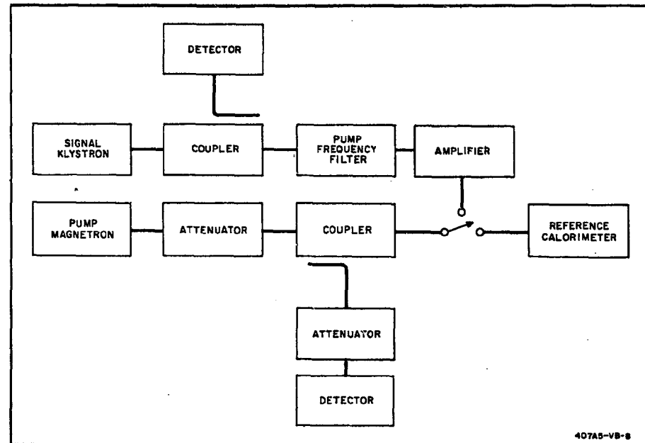
Figure 8. Pump-Signal Circuit
