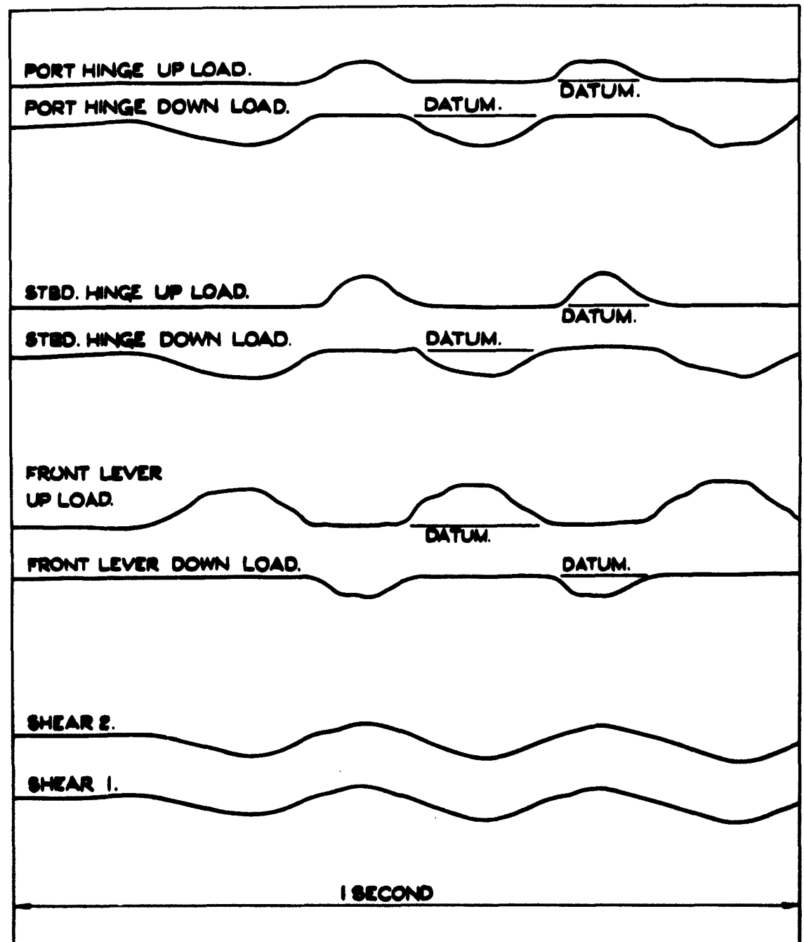
FIG. 10. TYPICAL LOAD RECORDS DURING IN-FLIGHT DATUM DETERMINATION.
