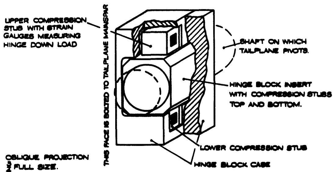
FIG 4(a) DIAGRAM OF HINGE BLOCK
