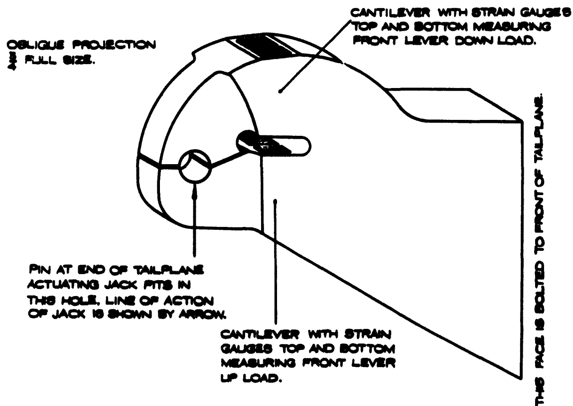
FIG. 4(b) DIAGRAM OF FRONT LEVER.
