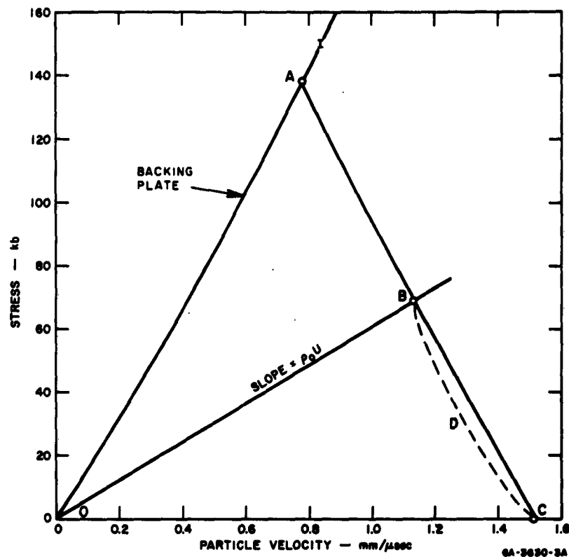
FIG. 3 IMPEDANCE MATCH SOLUTION
