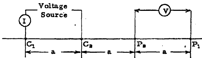
Figure 39. ELTRAN ARRAY.
