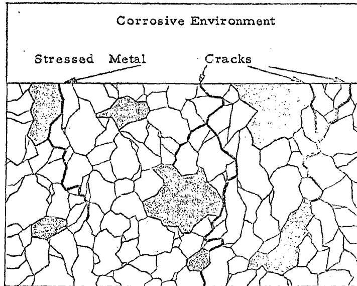
Figure 10. STRESS CORROSION.
