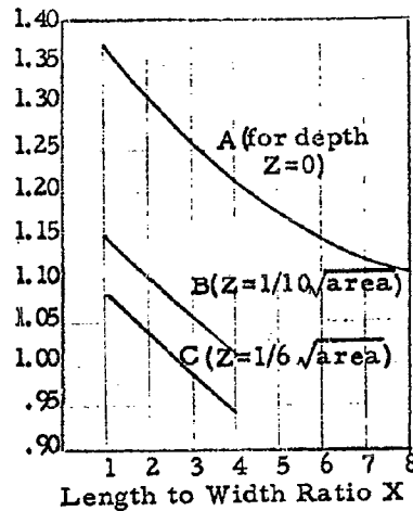
Figure 24. Values of Coefficient k_1 as function of length to width ratio X of of Area.
