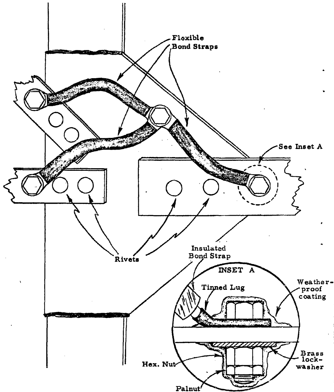
Figure 15.7. TECHNIQUES FOR BONDING METALLIC MEMBERS CONNECTED BY RIVETS.
