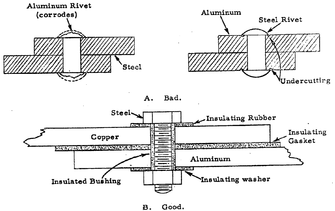
Figure 11. CONNECTION OF DISSIMILAR METALS.*
