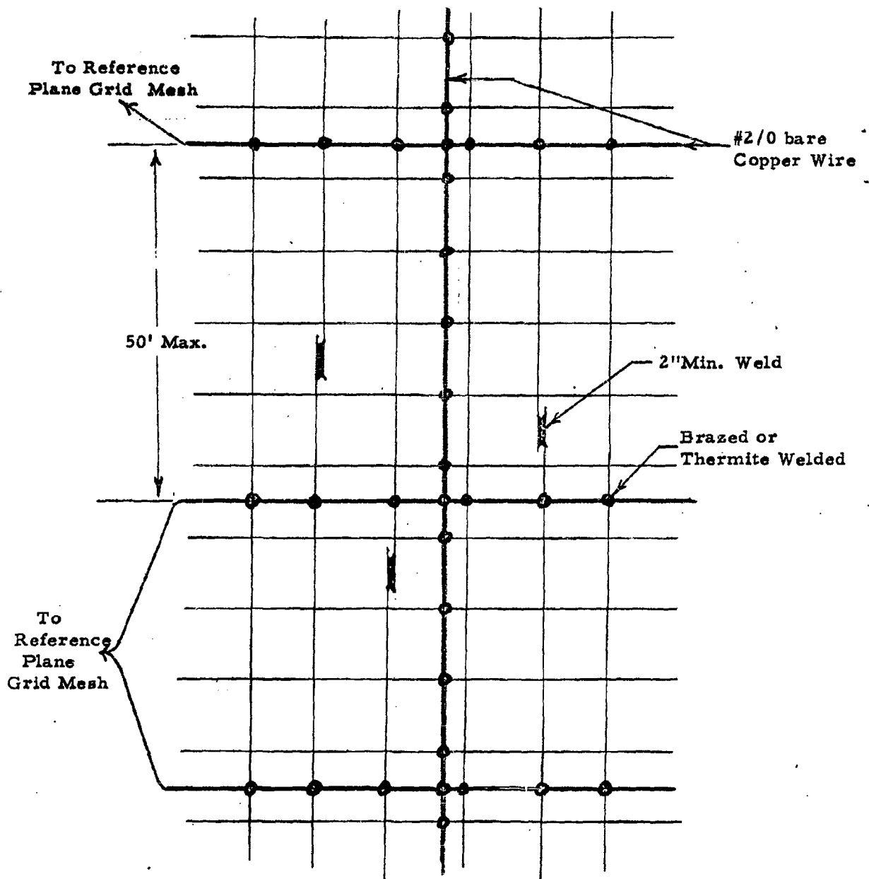
Figure 22. REINFORCEMENT BAR TIE-IN.
