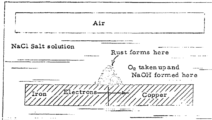
Figure 7. GALVANIC CORROSION.
