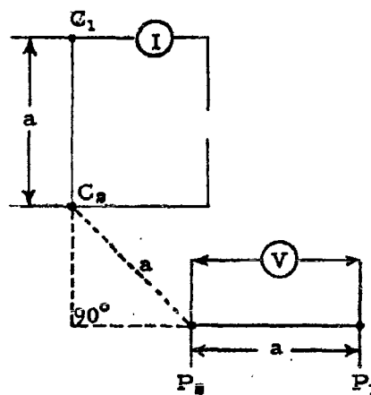
Figure 40. WAIT ARRAY.
