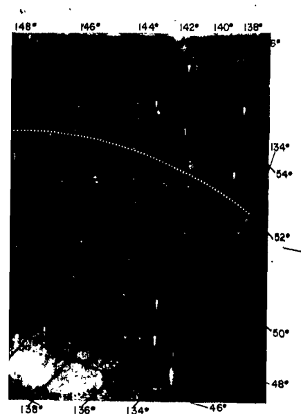
FRAME 1 0156.5 GMT 19 MAY 1960 DATA 0000 GMT 19 MAY 1960
