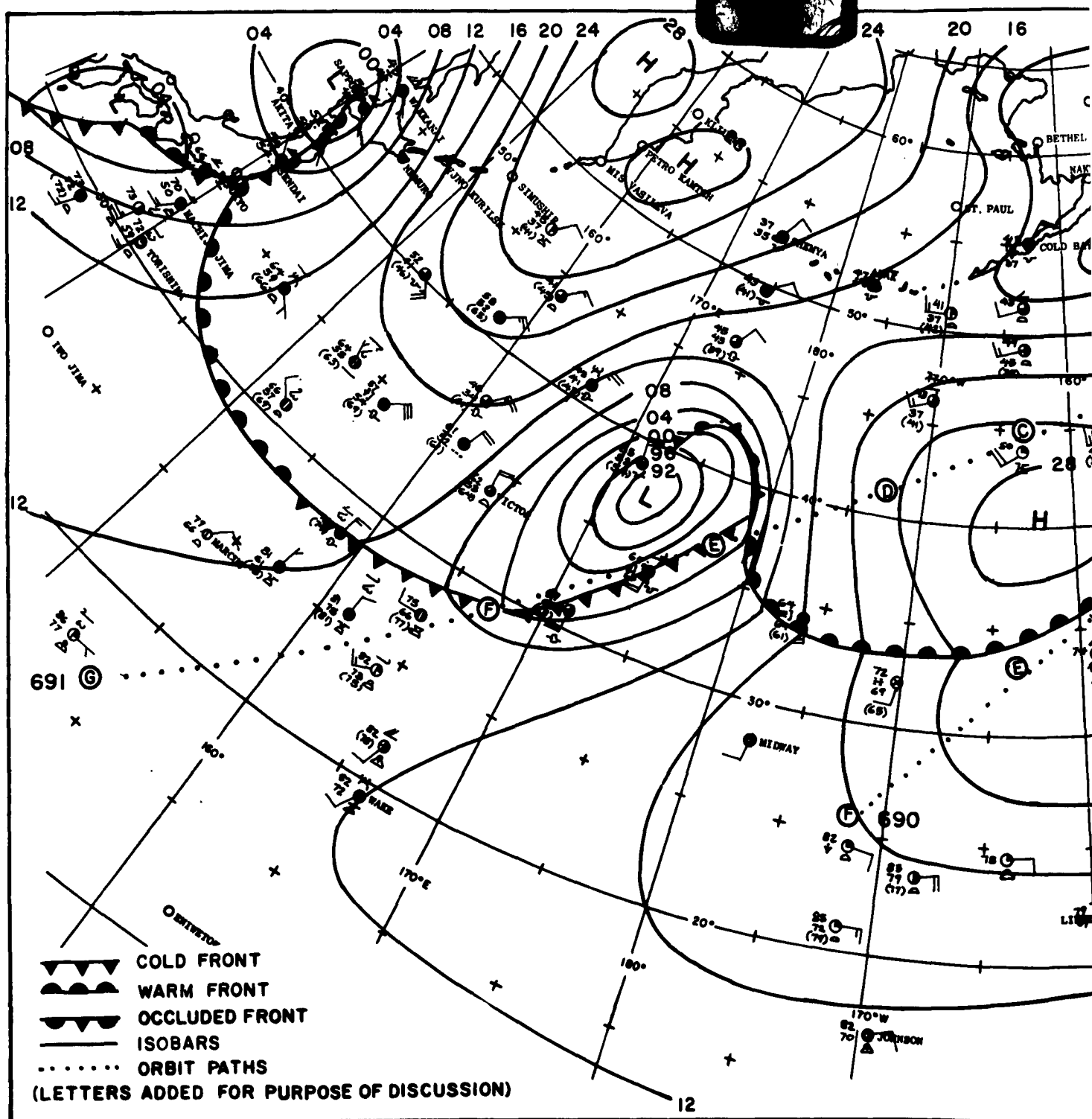
FIG. 6 SURFACE MAP, 19 MAY 11
