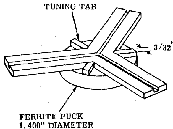
Figure 15. Sketch of 1.0 - 2.0 Gc Circulator with Tuning Tabs
