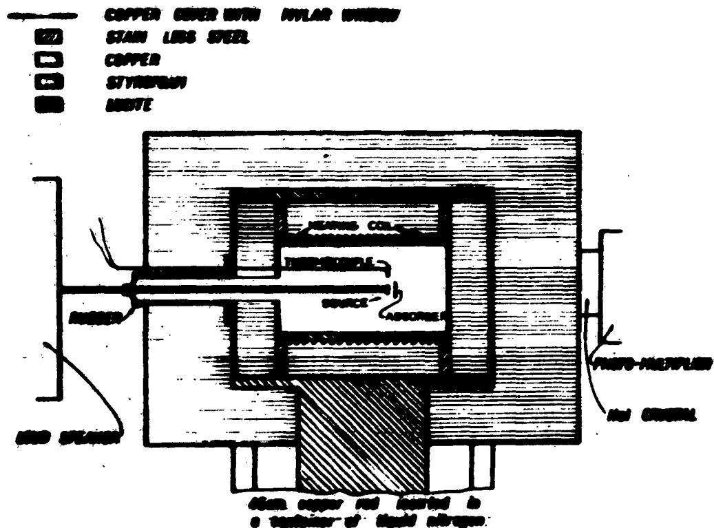
Fig. 2 Experimental arrangement for carrying out recoil-less absorption measurement with source and absorber at liquid nitrogen temperature.
