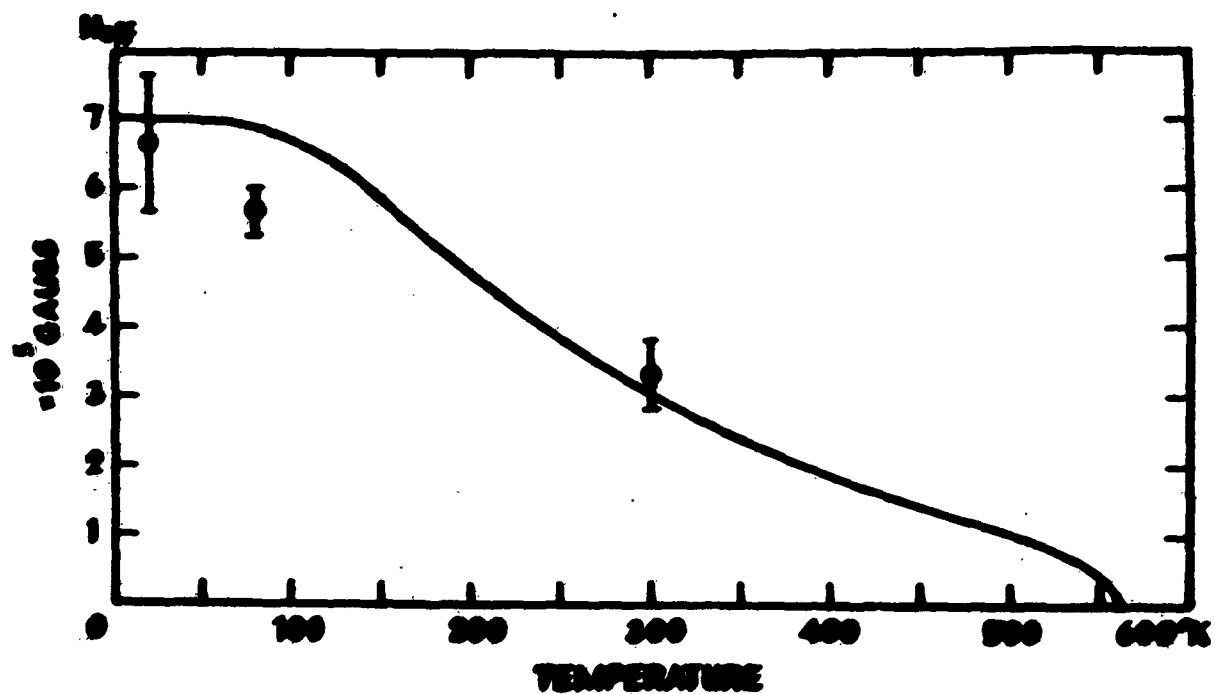
Fig. 8 Solid line represents the theoretical temperature dependence of H_{eff} action of the Eu nuclei in EuIG. Points represent the experimental values of H_{eff} obtained in the present work.
