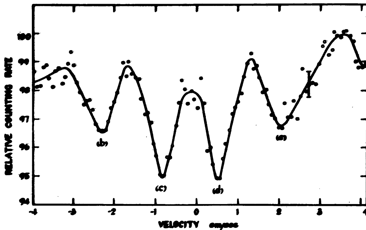
Fig. 5 The absorption by europium iron garnet at 81°K of the 21.7 kev \gamma -ray emitted in the decay of Gd^{151} , as a function of relative velocity between source and absorber. (Range of velocities -4 cm/sec to +4 cm/sec).
