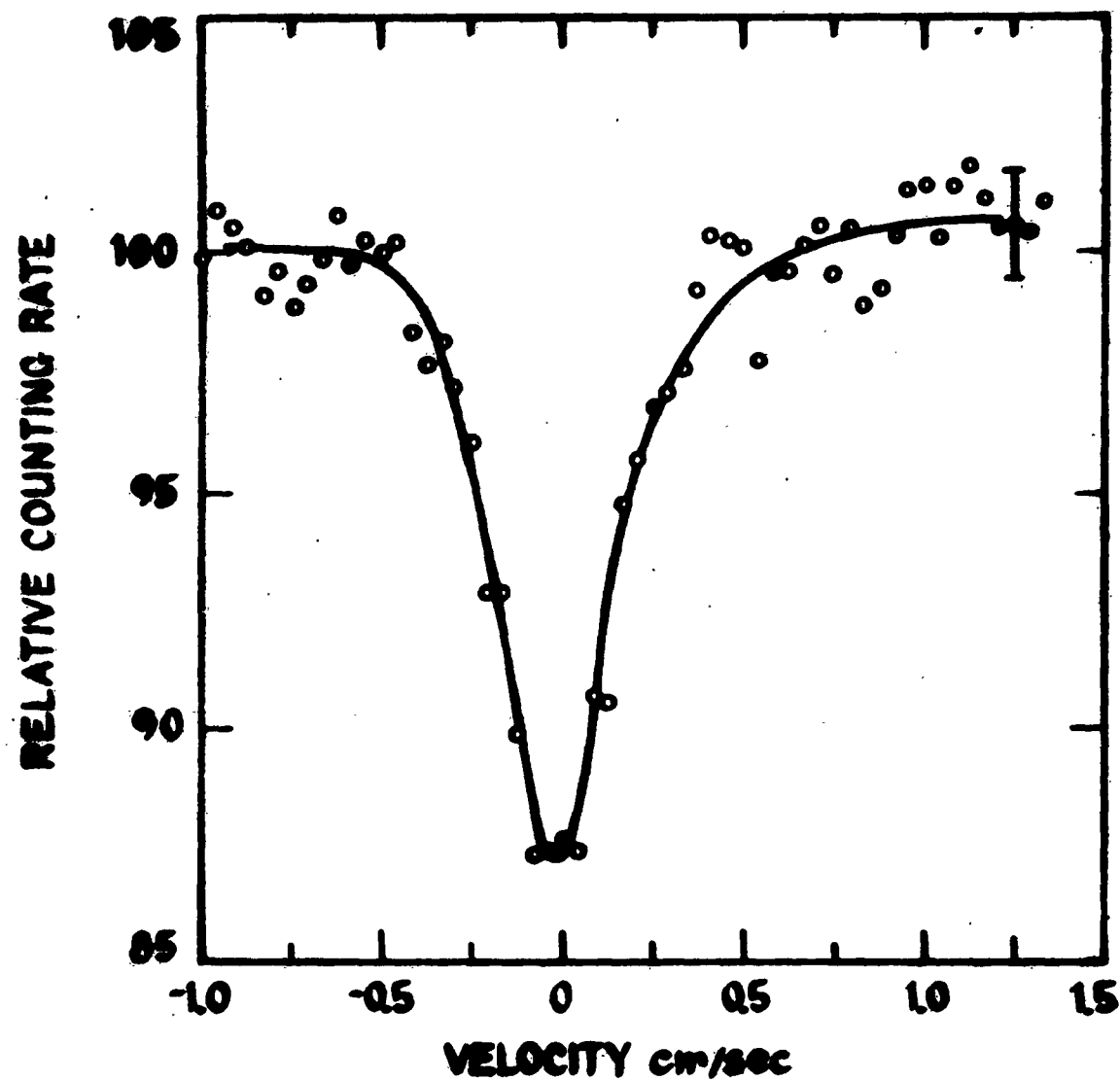
Fig. 3 The absorption by \text{Eu}_2\text{O}_3 at 81^\circ\text{K} of the 21.7 kev \gamma -ray emitted from an oxide source of \text{Gd}^{151} at 81^\circ\text{K} , as a function of relative velocity between source and absorber.
