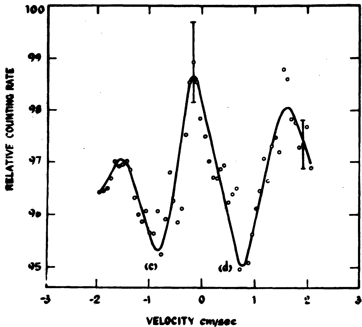
Fig. 7 The absorption by europium iron garnet at 20°K of the 21.7 kev \gamma -ray emitted in the decay of Gd^{151} , as a function of relative velocity between source and absorber.
