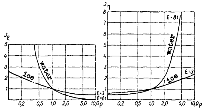
Figure 1. Relationship of the basic components of scattering energy to the shape factor \rho of water and ice particles. I_{\xi} is the component along the axis of rotation of the ellipsoid, I_{\eta} is the component in a perpendicular direction. The values of the scattered energy are given in fractions of the energy scattered by spherical particles of equivalent volume.
