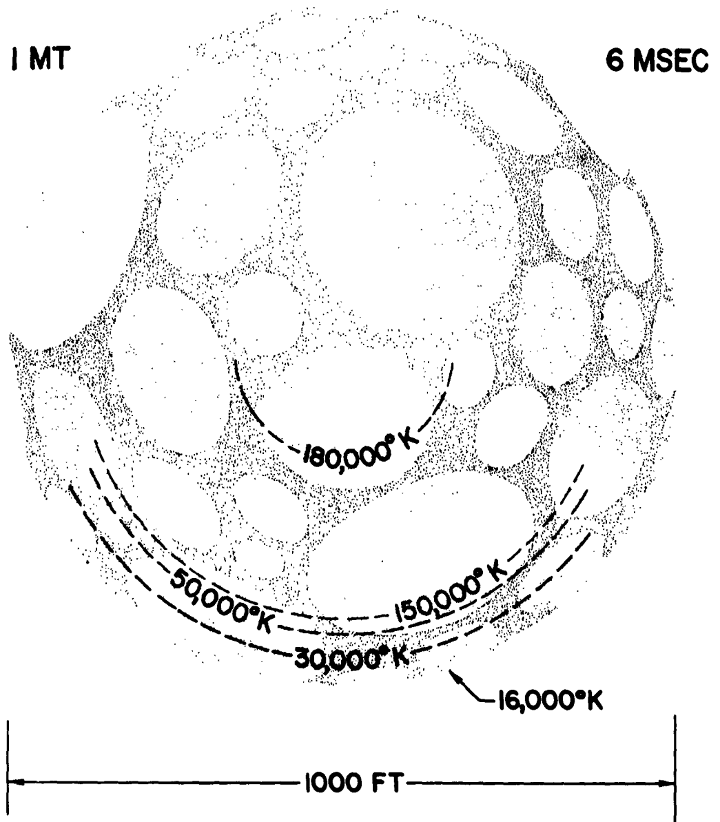
Fig.2---Early fireball size and temperature (while shock front is opaque)
