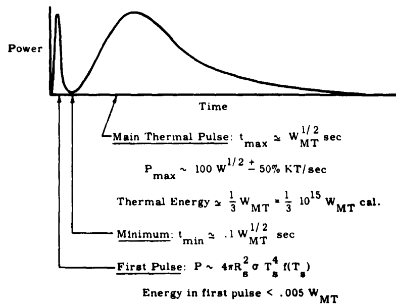
Fig.5---Thermal radiation rate versus time
