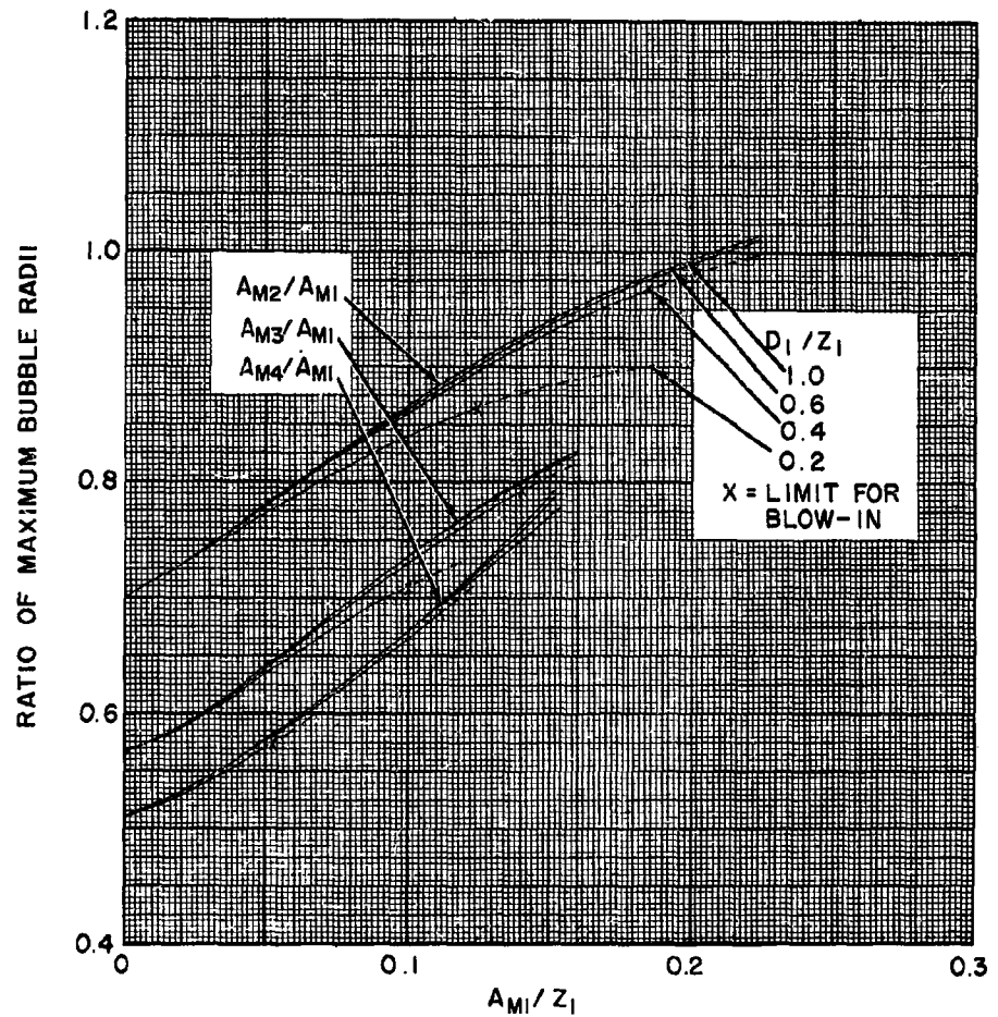
FIG. 7 RELATIVE MAXIMUM BUBBLE RADII
