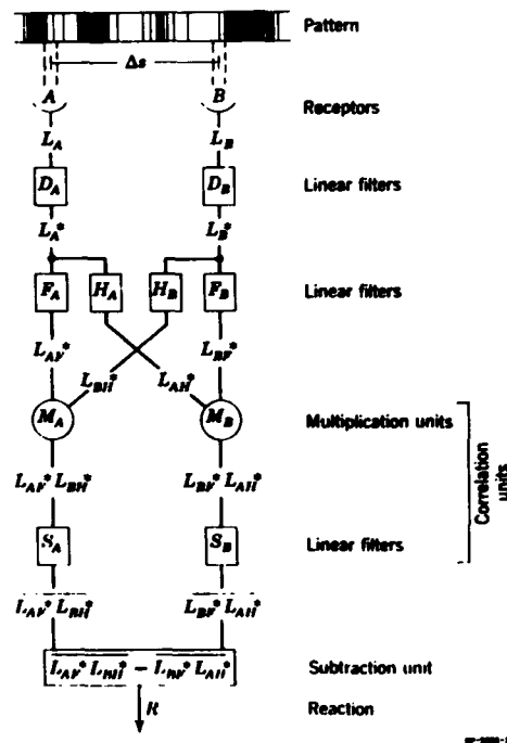
FIG. 7 REICHARDT'S MINIMAL MATHEMATICAL MODEL FOR A TWO-OMMATIDIA SYSTEM
