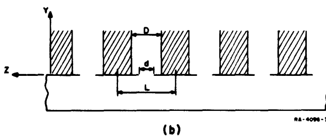
FIG. IV-2 WAVEGUIDE LEAKY-WAVE FILTER STRUCTURE (a) Orthogonal Projection (b) Longitudinal-Section View
