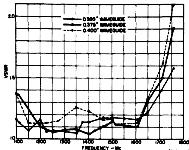
FIG. II-4 PASS-BAND VSWR OF SINGLE-LAYER WAFFLE-IRON FILTER WITH ROUND TEETH AND HALF-INDUCTIVE END-SECTIONS (Fig. II-1) OPERATING BETWEEN WAVEGUIDES OF VARIOUS HEIGHTS
