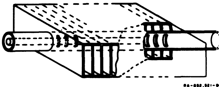
FIG. III-1 A COAXIAL LEAKY-WAVE FILTER FOR THE SUPPRESSION OF SPURIOUS ENERGY
