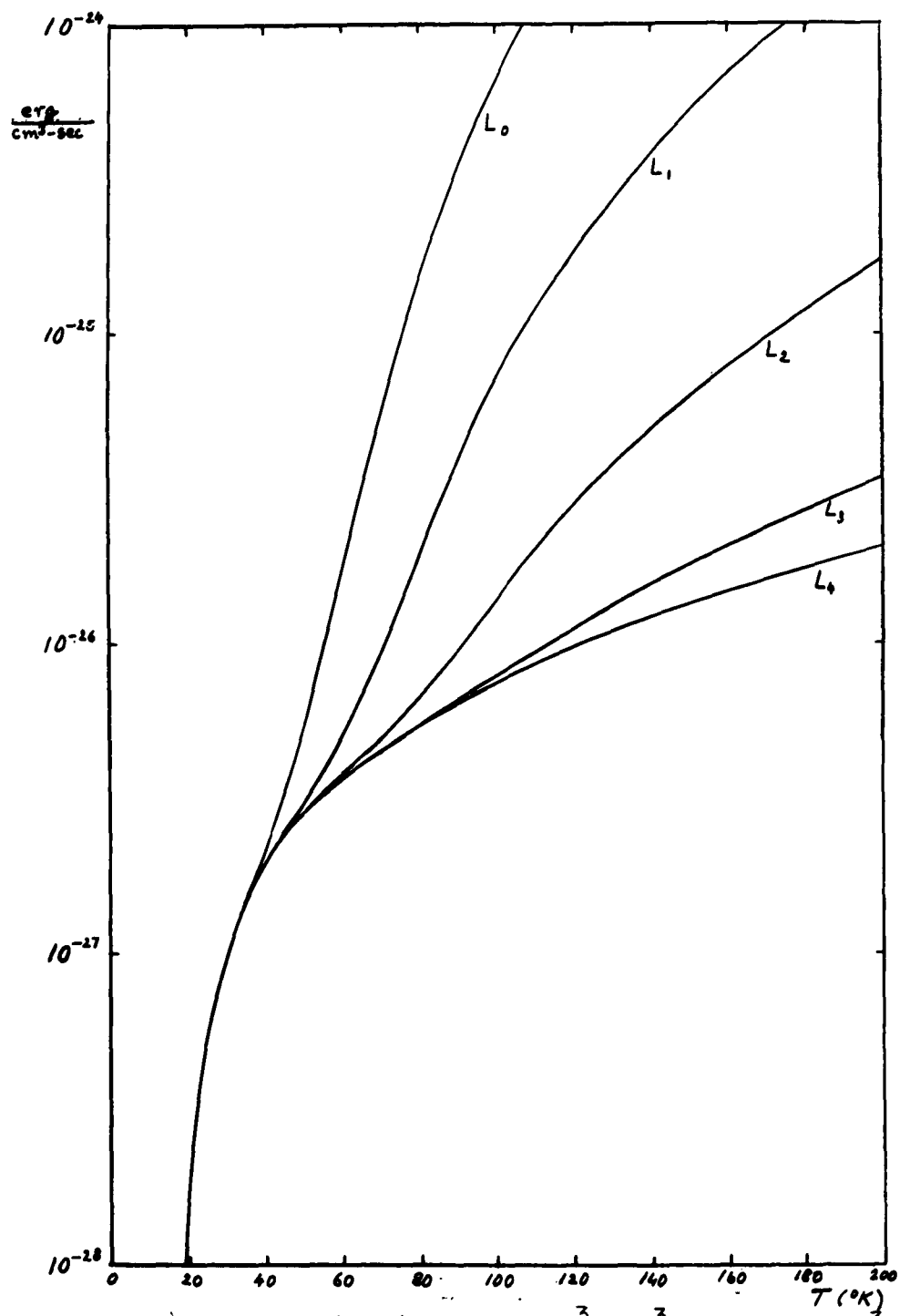
Fig. 33. L_p(T) for n_e = 2 \times 10^{-3} \text{ cm}^{-3} , n_H = 10 \text{ cm}^{-3} . p \equiv \log \frac{n_H}{n_{H_2}} .
