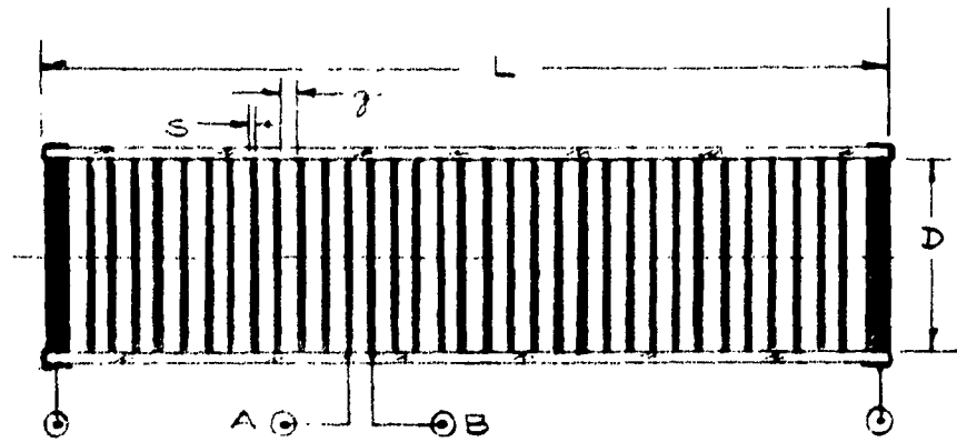
Fig. 1.4 - SPIRAL WINDING
