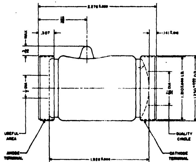
OUTLINE DRAWING ITT - Type 7177/1C - 6
