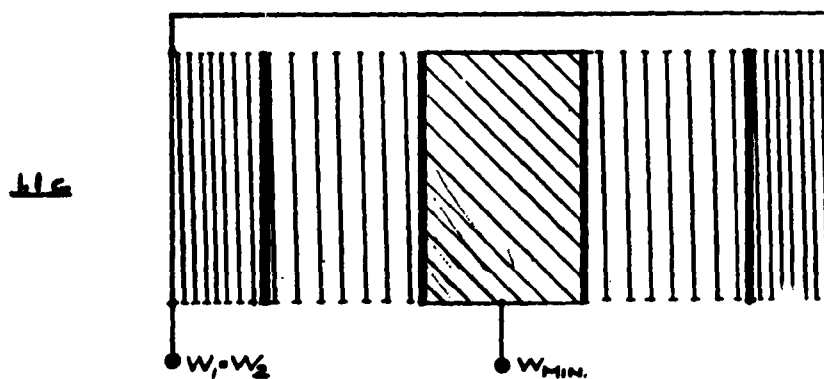
fig. 1.1 - SPIRAL LENS DESIGN: TWO-STEP APPROXIMATION
