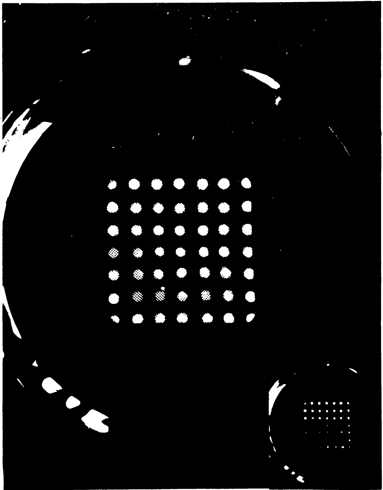
Fig. 4.6- IMAGE OBTAINED WITH CONVERTER TUBE OF Fig 4.4
