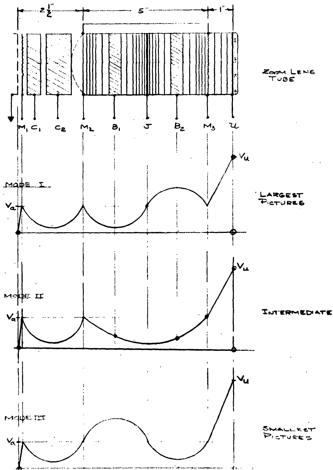
Fig. 5.2- SPIRAL ZOOM LENS
