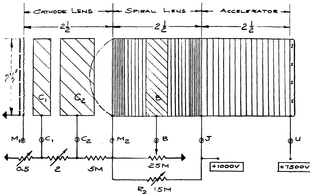
Fig. 4.1: SINGLE SPIRAL-LENS TUBE
