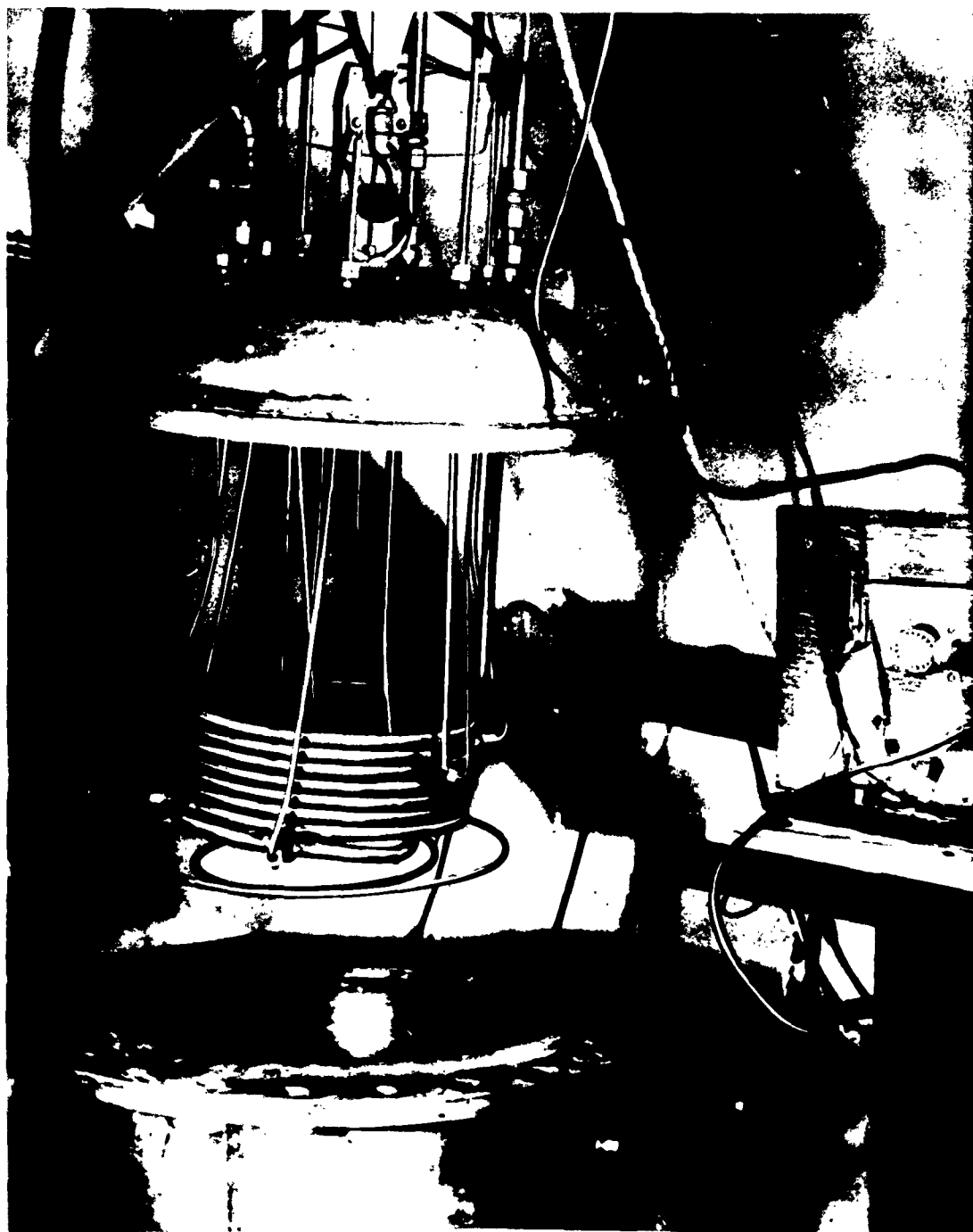
Fig. 9. Coiled tube and vacuum-jacketed vessel used in the pressure and temperature experiments.
