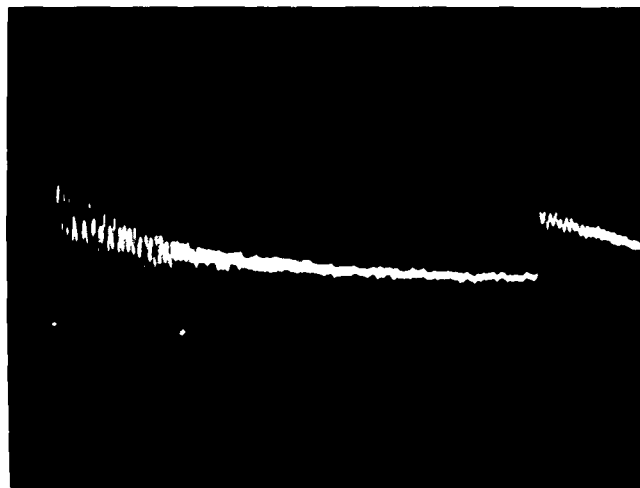
Fig. 8. Pressure trace of H_2-O_2 detonation wave in straight tube using the Kistler Model 603 pressure transducer.
