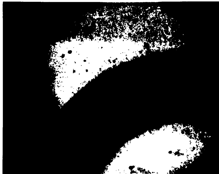
Fig. 14. Spark-schlieren photographs at different magnifications of two 60%, H_2-O_2 detonation waves passing through the curved test section.
