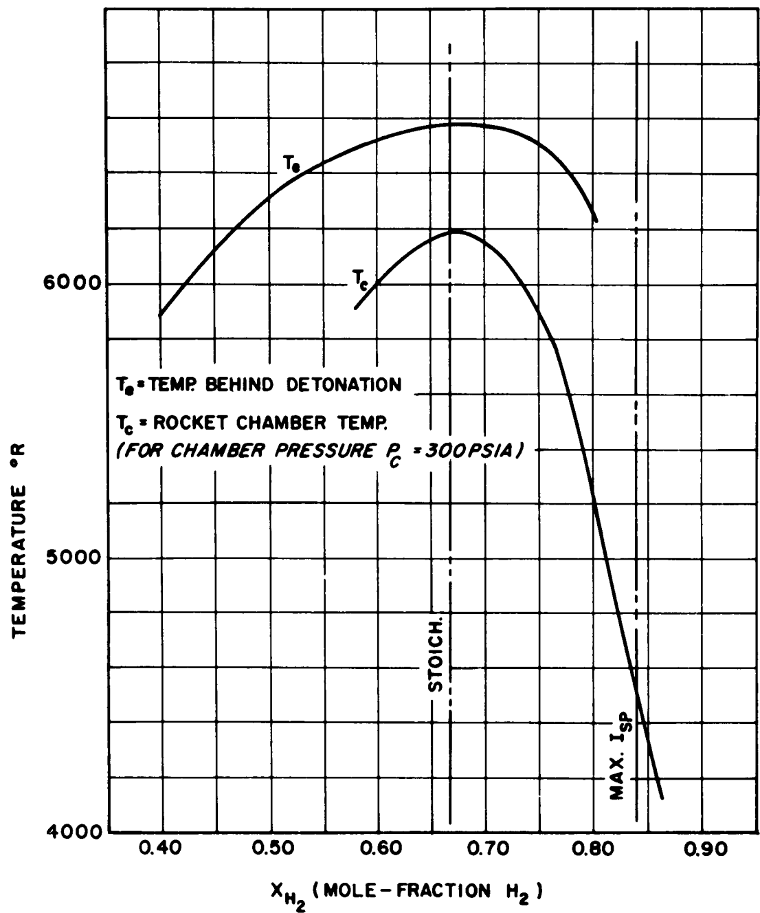
Fig. 3. H_2 - O_2 Chapman-Jouguet detonation and combustion chamber temperatures as a function of mixture ratio.
