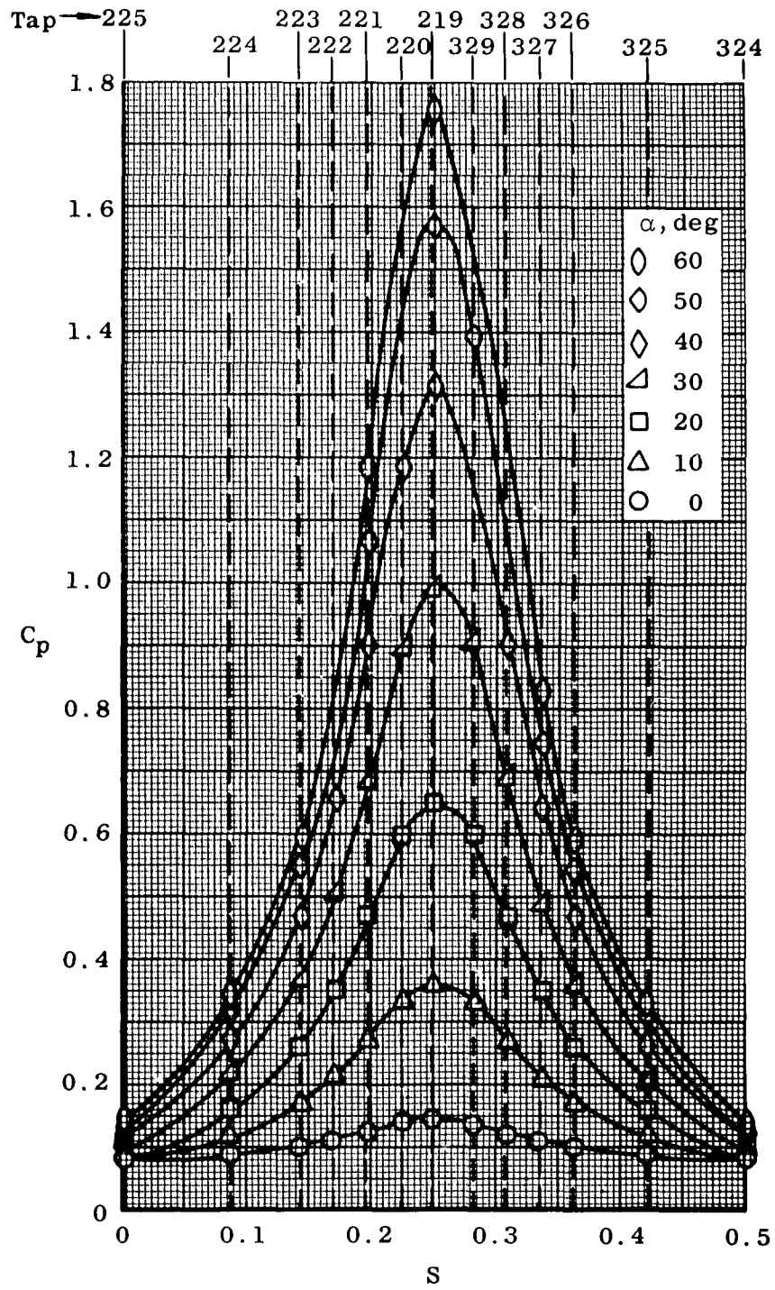
Fig. 16 Pressure Distribution for Cross Section 11.5 of Configuration 2
