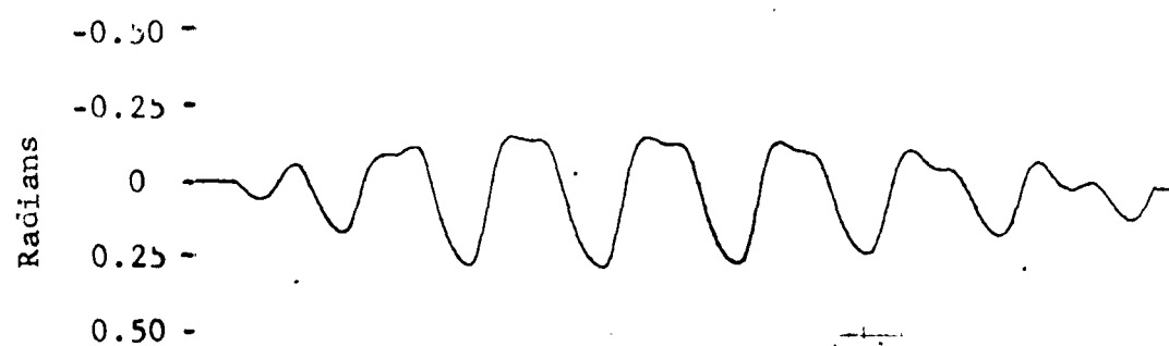
(c) Stable Solution, \omega = 7.02 rad/sec
