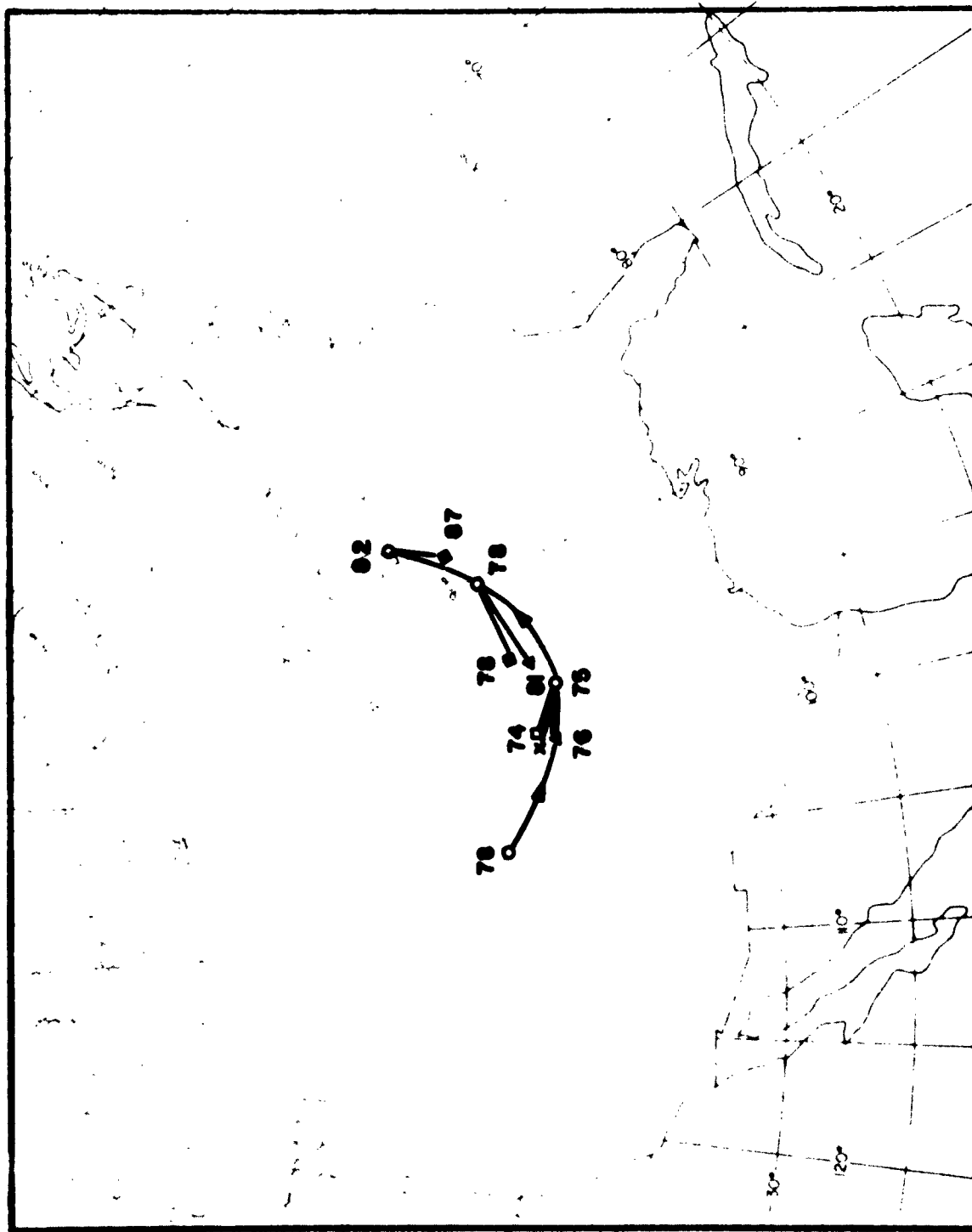
Fig. 8-6(b). Forecast verification. \circ observed, \square base technique, \triangle surface predictors only, \times modified technique; adjacent numerals indicate central pressure.
