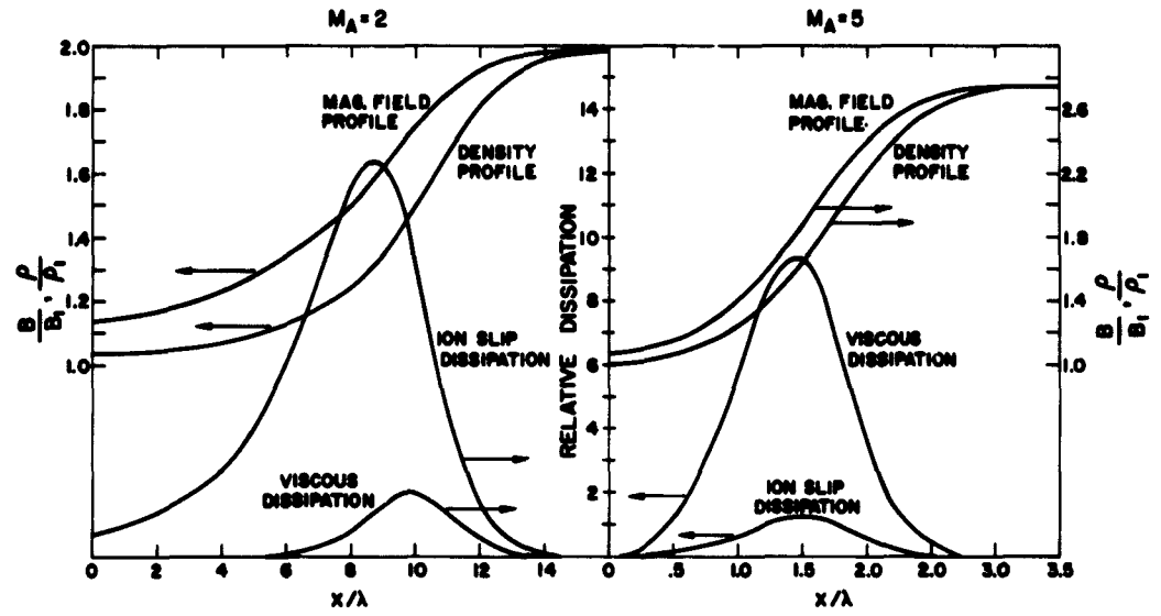
Fig. 3 The magnetic field and density shock profiles are shown for two Mach numbers; one where the dissipation is largely ion slip ( J \cdot E ) and the other where the dissipation is largely \mu(du/dx)^2 . The dissipation rates are suitably nondimensionalized.
