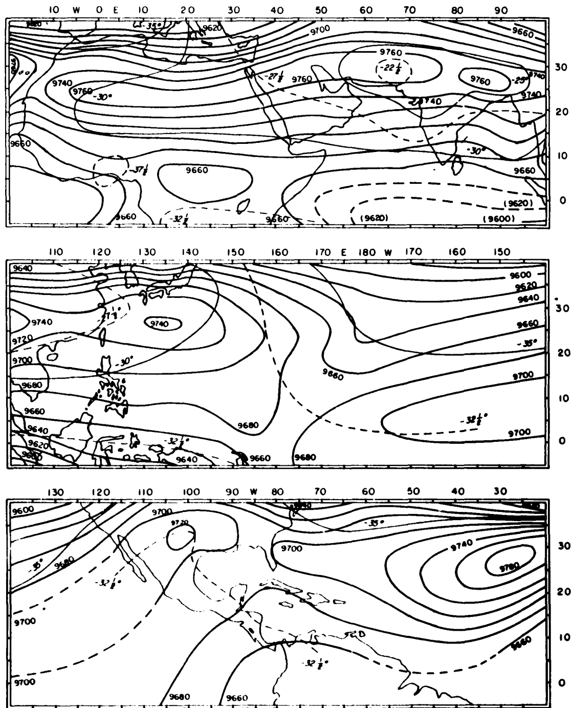
MEAN JULY CONTOUR HEIGHTS AND TEMPERATURES, 300mb
