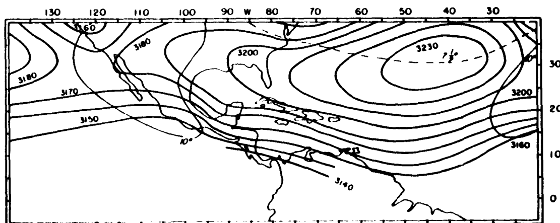
MEAN JULY CONTOUR HEIGHTS AND TEMPERATURES, 700 mbs
