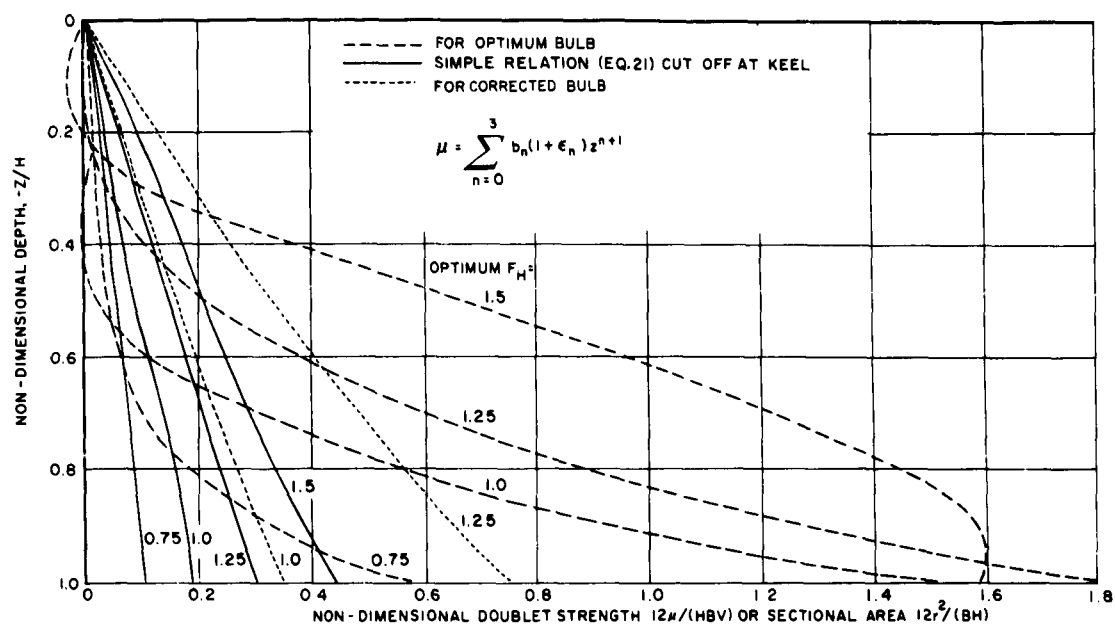
FIGURE 1a DOUBLET DISTRIBUTION FOR SINE SHIP ( L/H=16 )
