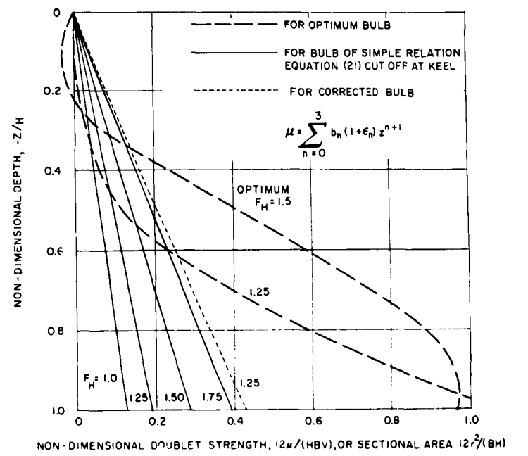
FIGURE 2a- DOUBLET DISTRIBUTION FOR SINE SHIP ( L/H = 24 )
