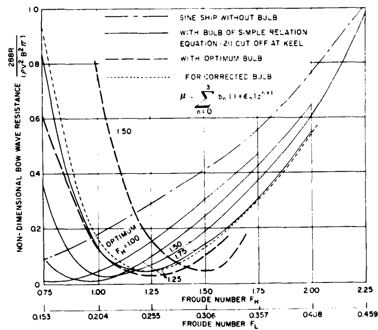
FIGURE 2b- BOW WAVE RESISTANCE OF SINE SHIP ( L/H = 24 )
