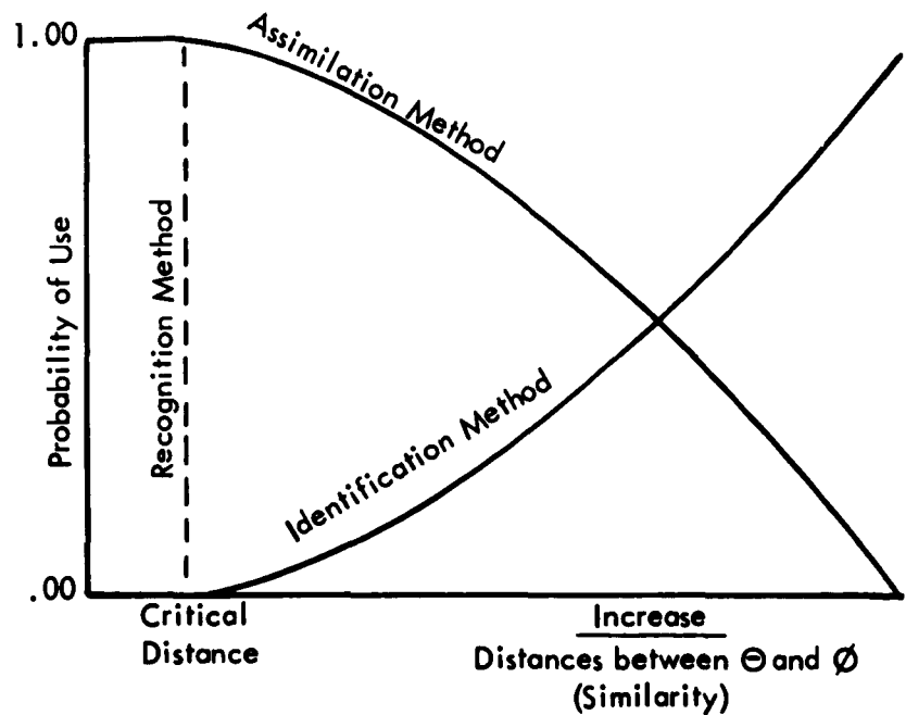
Fig. 2. Probability of use of each inference method as a function of the distance between \Theta and \emptyset .
