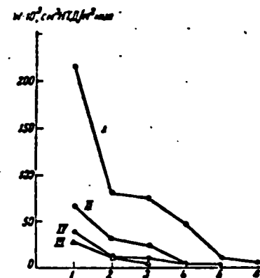
Fig.7. Rate of decomposition of hydrazine on copper polychelates, characterized by composition of chelate unit, in relation to composition or organic radical of polymers:
