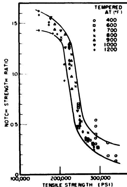
Fig. 6 - Notch strength ratio vs tensile strength for specimens tempered as indicated (tensile strengths from Ref. 7)
