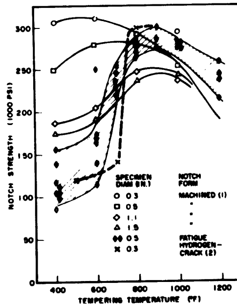
Fig. 13 - Comparative notch strength measurements as a function of tempering temperature for specimens of various sizes notched in the indicated ways
