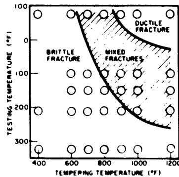
Fig. 8b - Suggested fracture transition behavior in 4340 steel as a function of tempering and testing temperatures
