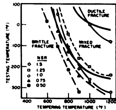
Fig. 9 - Contours of constant notch strength ratio superimposed on the fracture appearance field of Fig. 8b
