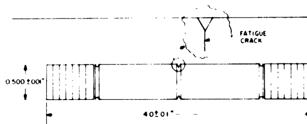
Fig. 2 - The notch-fatigue specimen in the final form for tension testing
