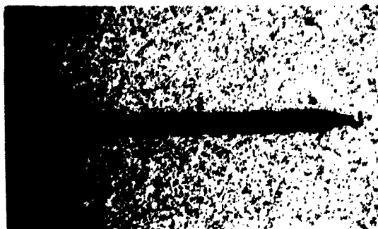
Fig. 11 - Opening of the fatigue crack 4340 steel specimen tempered at 1200°F, tested at 75°F
