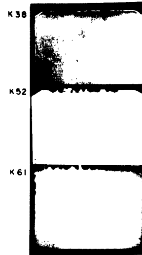
Fig. 12 - Photomicrographs illustrating crack development normal to the plane of the primary fracture (~X5): specimen K 38 tempered at 800°F, tested at 75°F; specimen K 52 tempered at 900°F, tested at 75°F; specimen K 61 tempered at 1000°F, tested at 75°F
