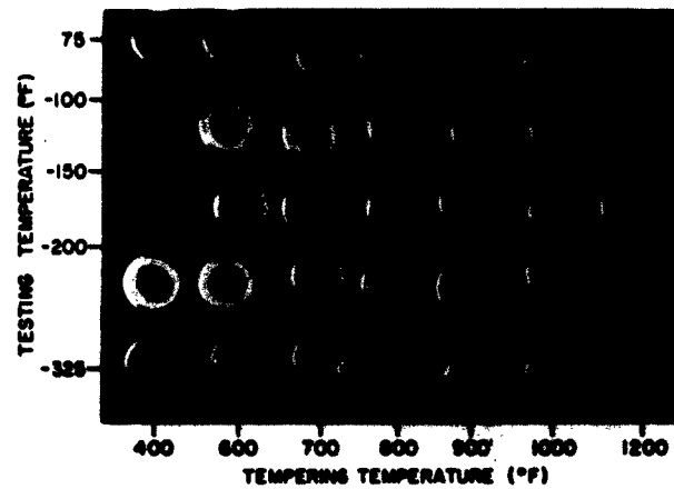
Fig. 8a - Characteristic fractures for fatigue-notch 4340 steel specimens as a function of tempering and testing temperatures
