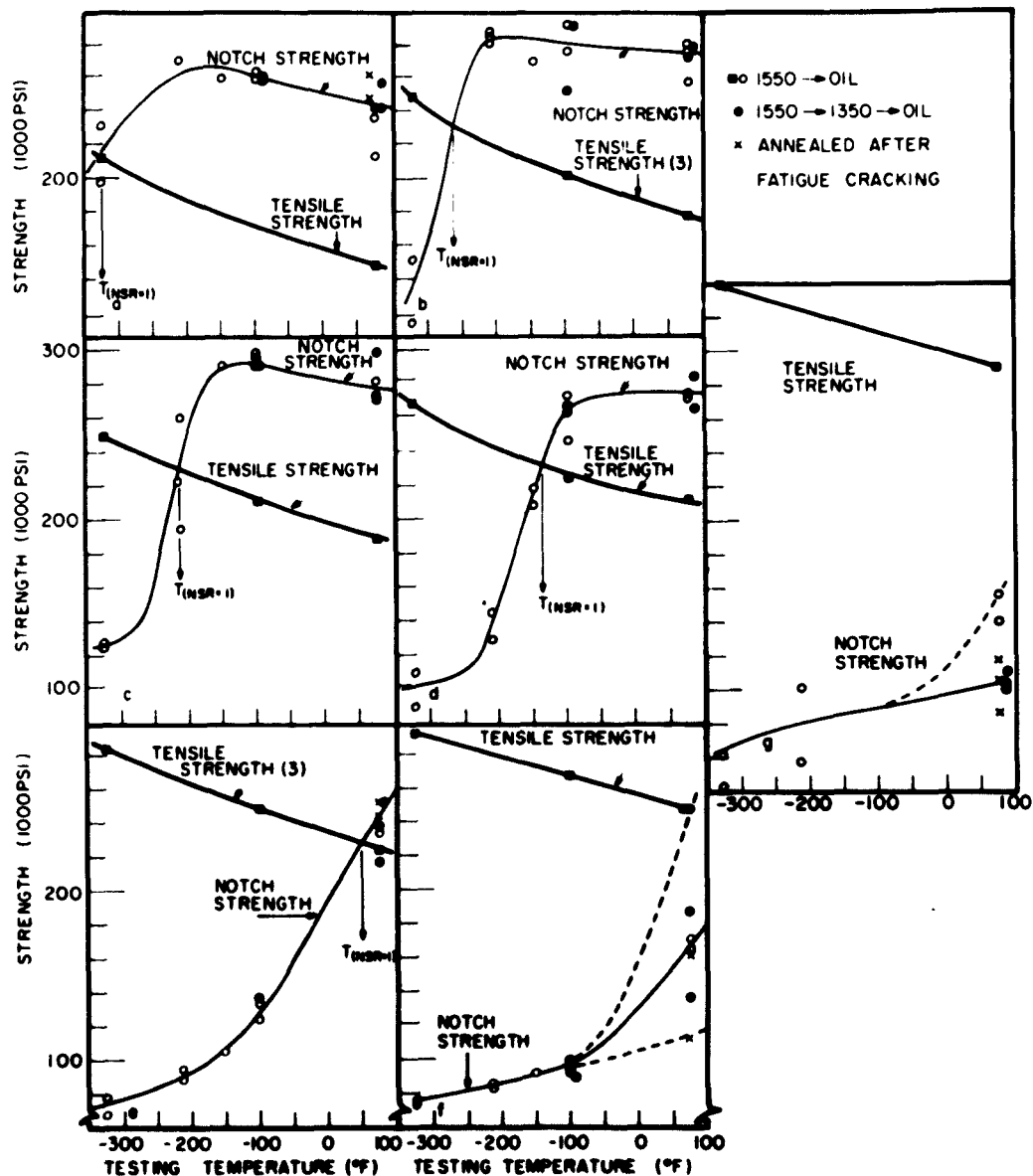
Fig. 4 - Tension and notch-tension data as a function of testing temperature with the tempering temperature as a parameter for 4340 steel (tensile strength from Ref. 7): (a) tempered at 1200°F 2 + 2 hours; (b) tempered at 1000°F 2 + 2 hours; (c) tempered at 900°F 2 + 2 hours; (d) tempered at 800°F 2 + 2 hours; (e) tempered at 700°F 2 + 2 hours; (f) tempered at 600°F 2 + 2 hours; (g) tempered at 400°F 2 + 2 hours
