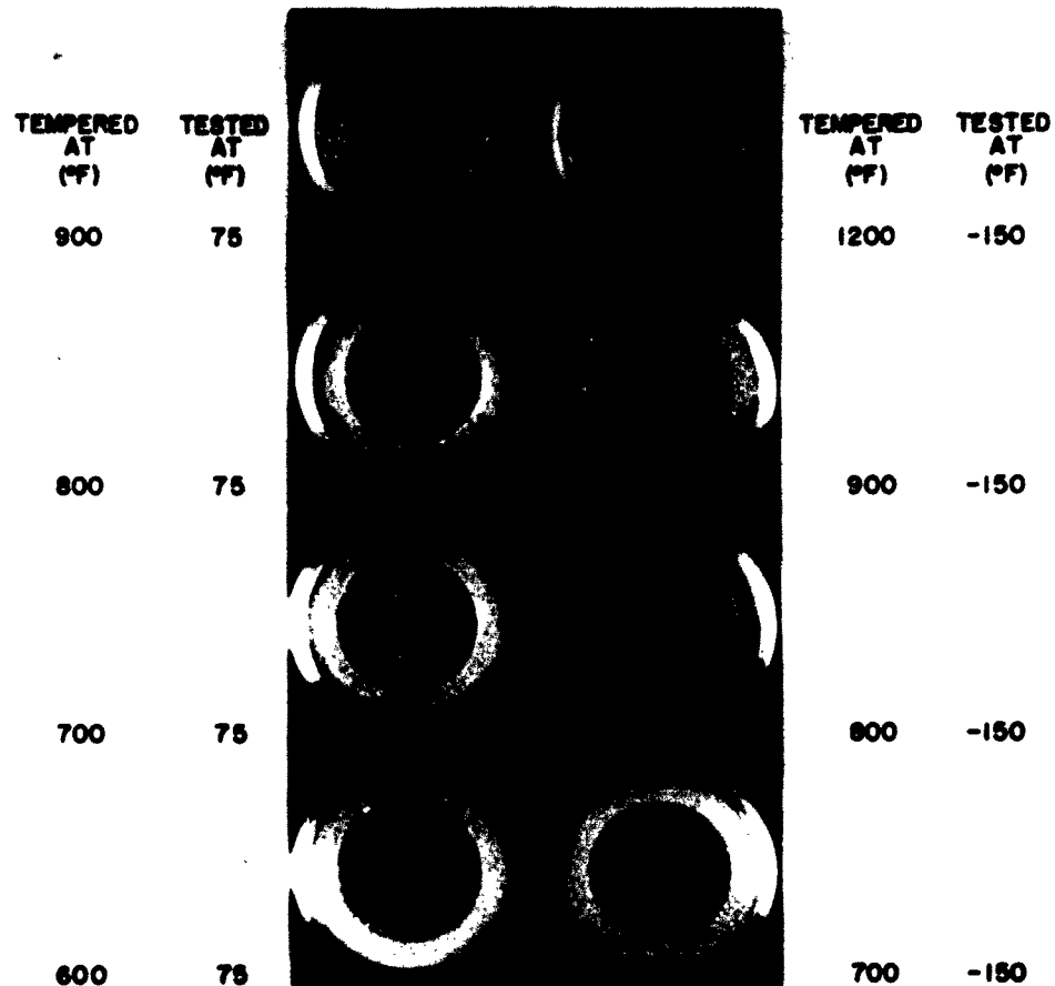
Fig. 10 - Fractographs illustrating the transition in fracture type with an increase in the strength level ( \sim X5 )
