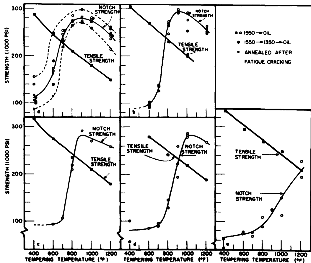
Fig. 5 - Tension and notch-tension data as a function of tempering temperature with the testing temperature as a parameter for 4340 steel (tensile strength from Ref. 7): (a) tested at 75^{\circ}\text{F} ; (b) tested at -100^{\circ}\text{F} ; (c) tested at -150^{\circ}\text{F} ; (d) tested at -200^{\circ}\text{F} ; (e) tested at -323^{\circ}\text{F}
