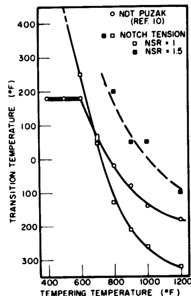
Fig. 7 - Transition temperatures for 4340 steel by the indicated notch-property criteria as a function of tempering temperature
