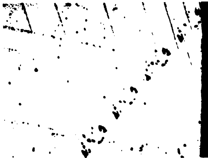
Figure 16 1000X Micro-cracks in twins in iron single crystal.
