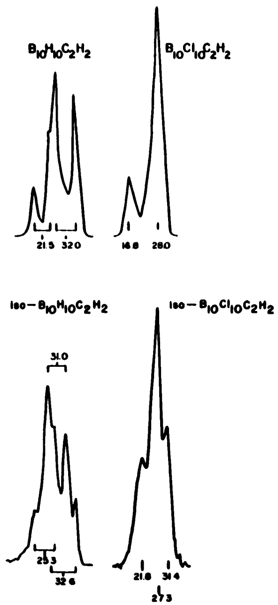
Fig. 2-11 ^{11}B n.m.r. spectra of two carboranes and two iso-carboranes in acetonitrile in displacement (in p.p.m.) from methyl borate. The chemical shifts of the boron resonance doublets were obtained from the decoupled spectra.
