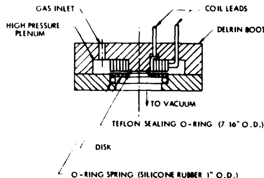
Fig. XII-12. Magnetically driven gas valve.
