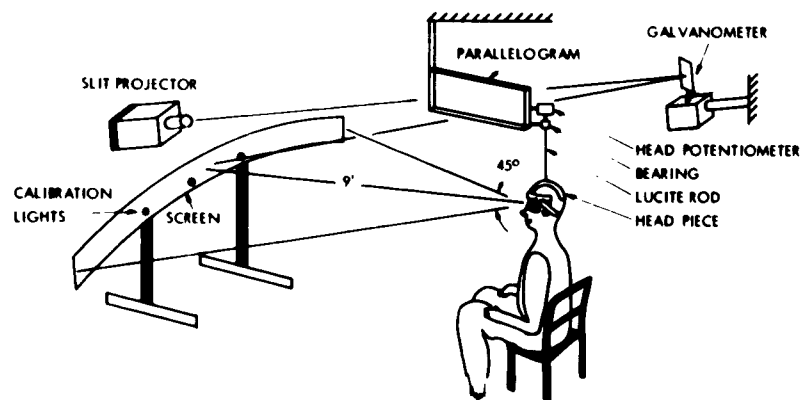
Fig. XXII-7. Relative positions of major apparatus.
