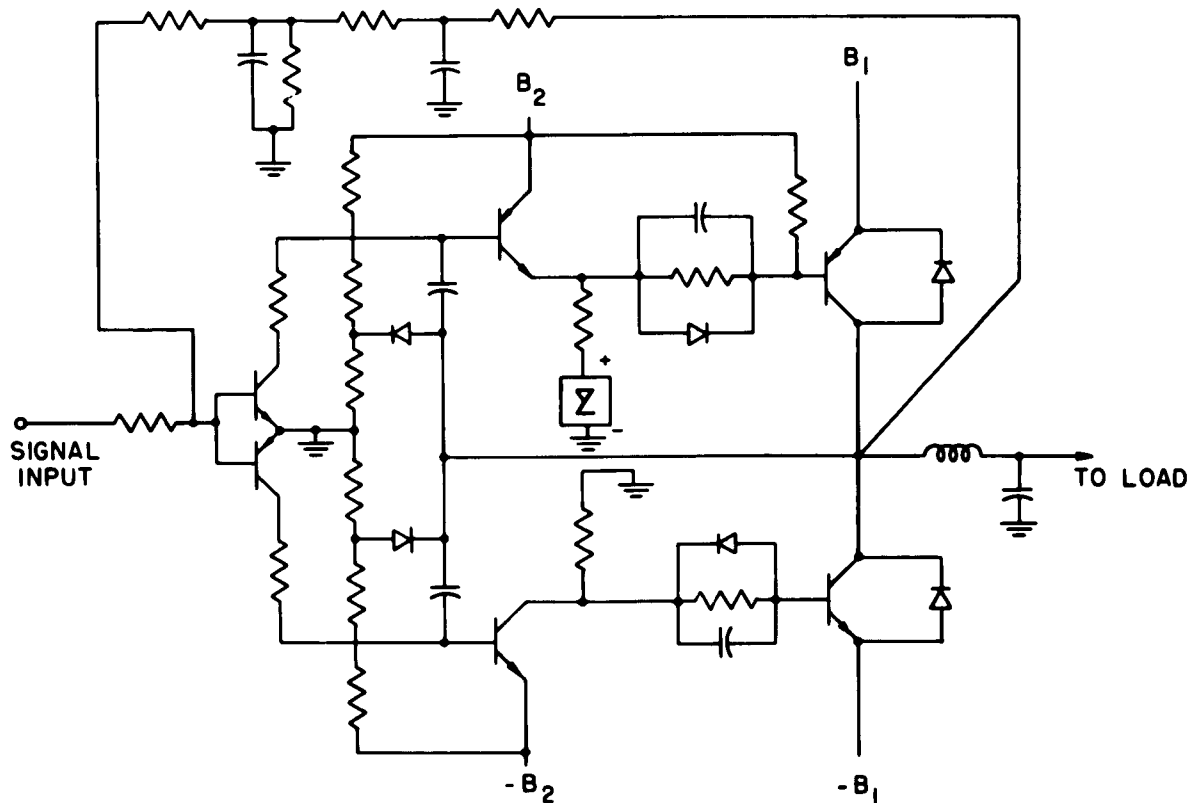
Fig. XIV-9. Circuit of 15-watt power amplifier.
