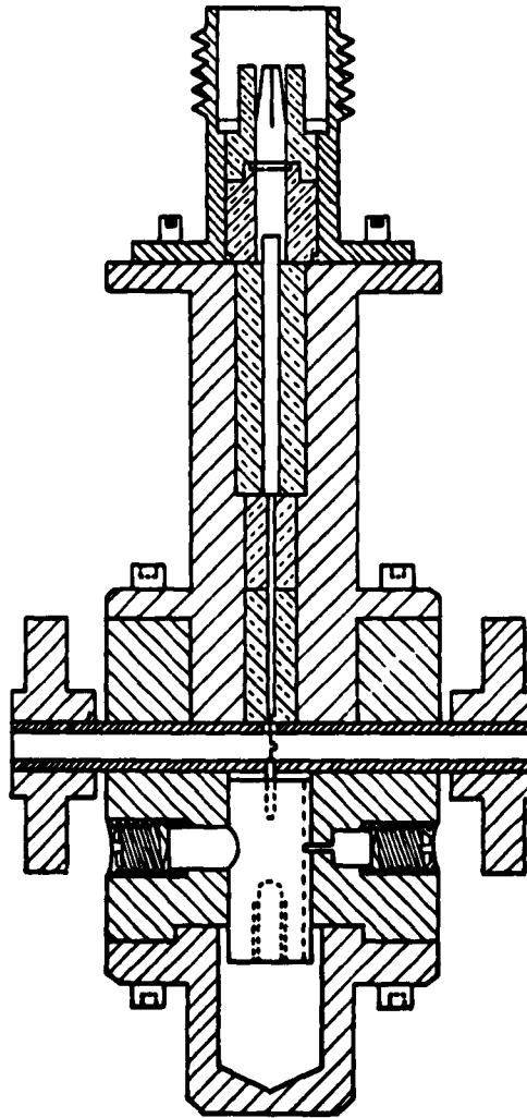
Fig. VII-5. Mixer assembly.
