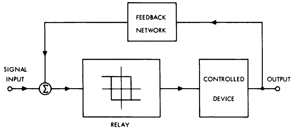
Fig. XIV-5. Simple relay servomechanism.
