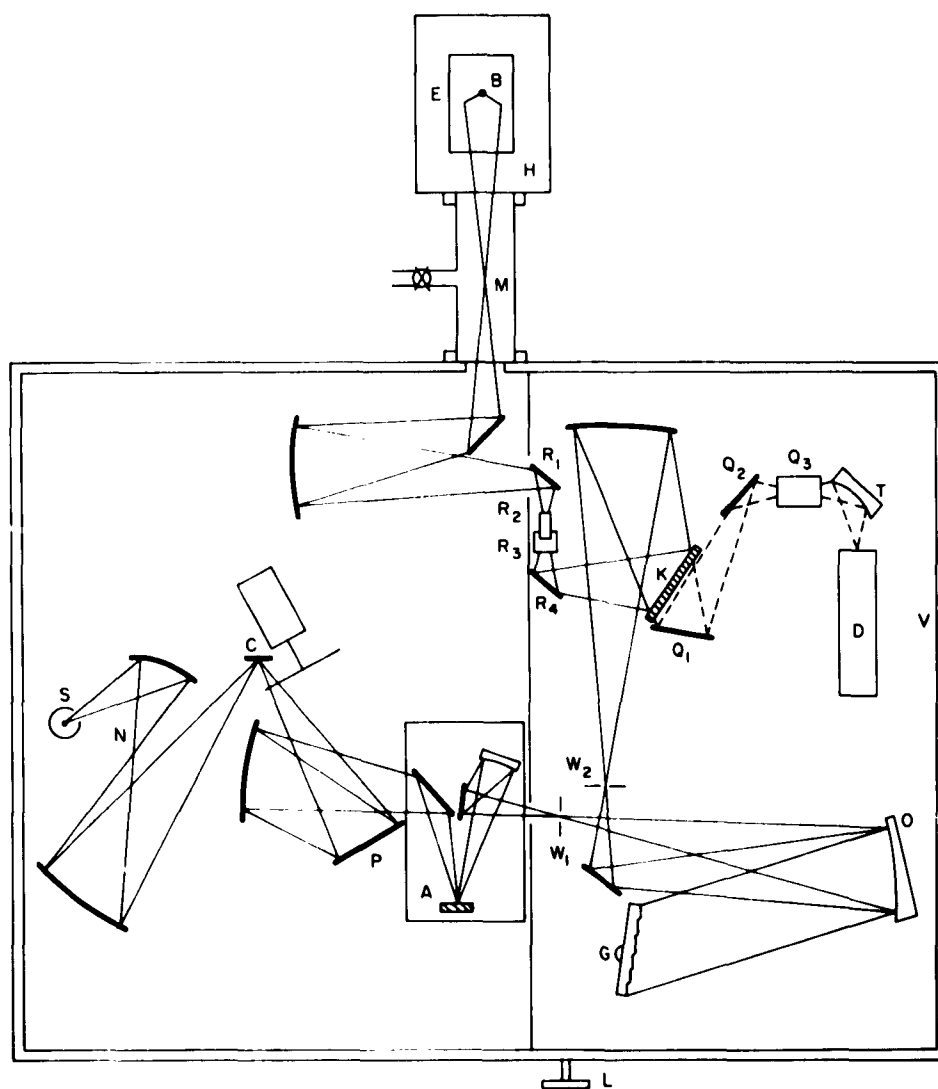
Fig. III-1. Optical layout of the far infrared spectrometer.
