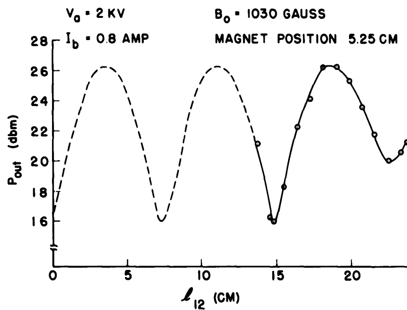
Fig. V-7. Second-cavity power output vs distance between cavity gaps for the cylindrical-cathode gun. (Cavity 1, P_{in} = 20 \text{ dbm.} )
