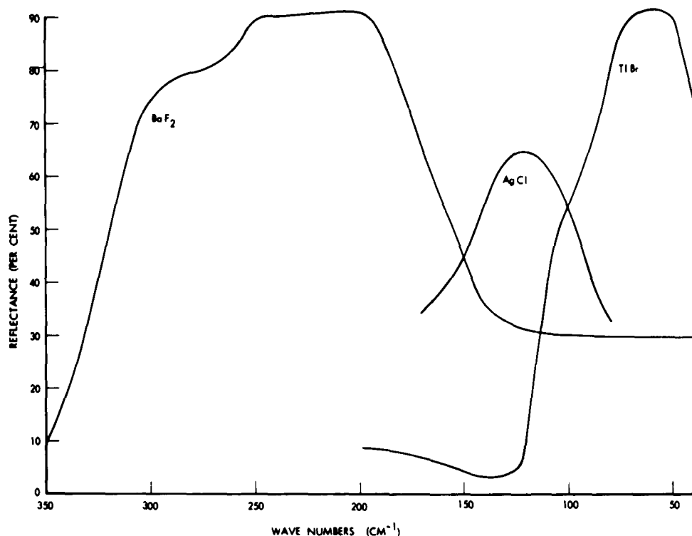
Fig. III-8. Reflectance curves for BaF 2 , AgCl, and TlBr.
