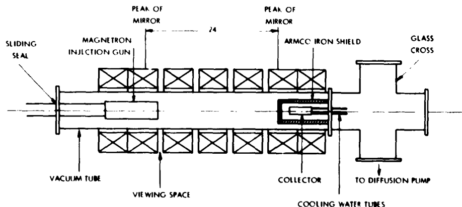
Fig. XII-11. Top view of hollow-beam experimental apparatus.
