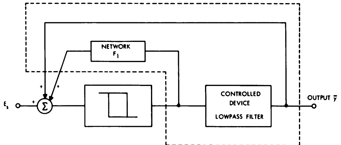
Fig. XIV-6. Nonlinear control system incorporating the modulator principle.
