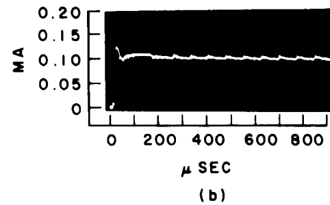
Fig. XII-37. Collected ion currents. V_I = 600 volts, V_{Acc} = 100 volts, V_N = 0 . Transit time, 22 \mu\text{sec} . (a) No electrons: rise time, \sim 500 \mu\text{sec} . (b) With electrons: rise time, \sim 25 \mu\text{sec} .
