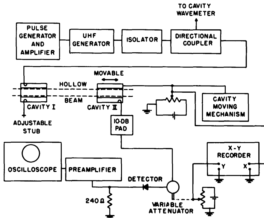
Fig. V-6. Space-charge wavelength, gain and noise measurement.
