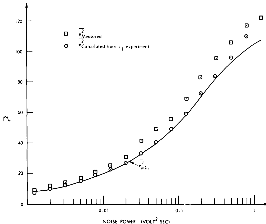
Fig. XIV-17. \overline{e^2}_{\text{measured}} , \overline{e^2}_{\text{minimum}} and \overline{e^2}_{\text{calculated from } x_i \text{ experiment}} versus noise power for S_0 = 0.79 \text{ volt}^2 \text{ sec} .
