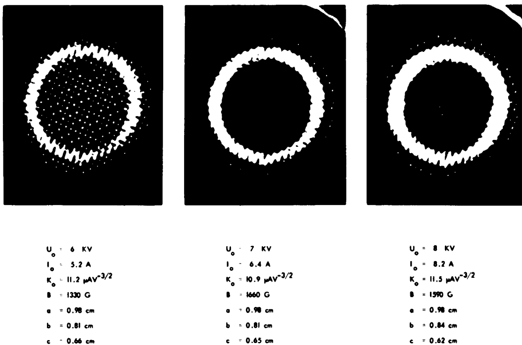
Fig. V-3. Hollow-beam cross sections.
