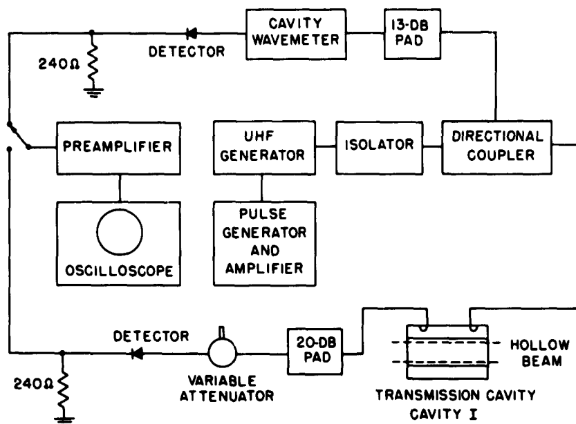
Fig. V-5. Beam-loading measurement.
