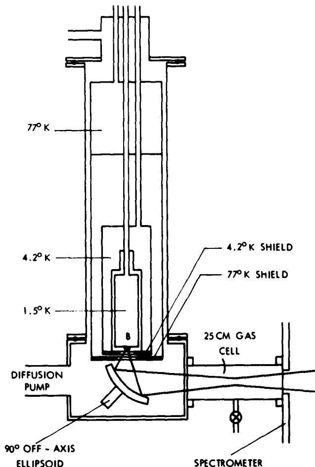
Fig. III-4. Detector optics and cryostat assembly.
