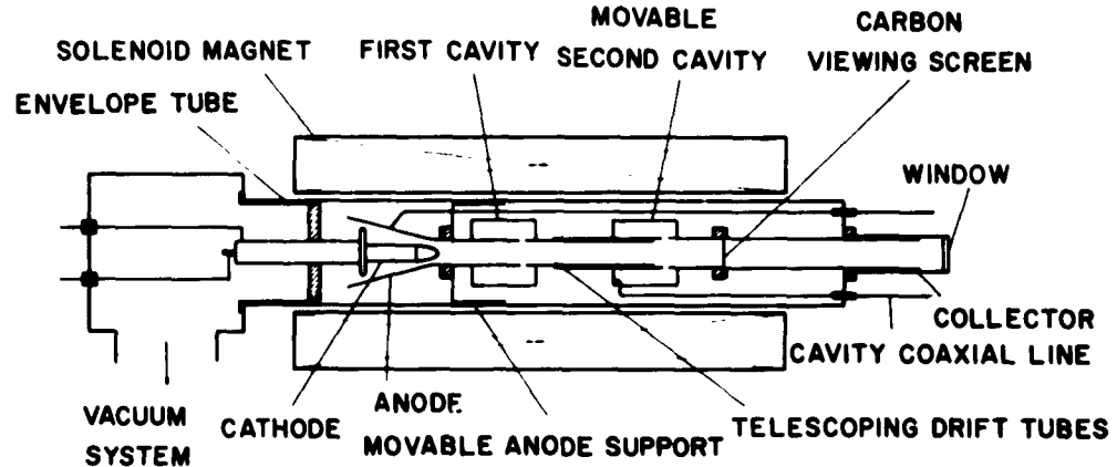
Fig. V-1. Schematic diagram of the beam tester.
