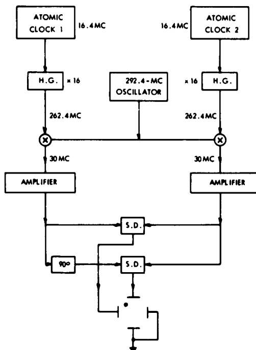
Fig. VI-1. Stability measurement system.
