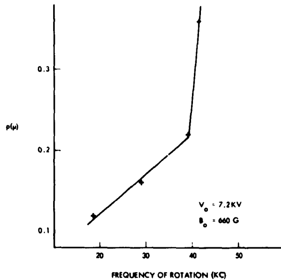
Fig. XII-9. Rotational frequency vs pressure.
