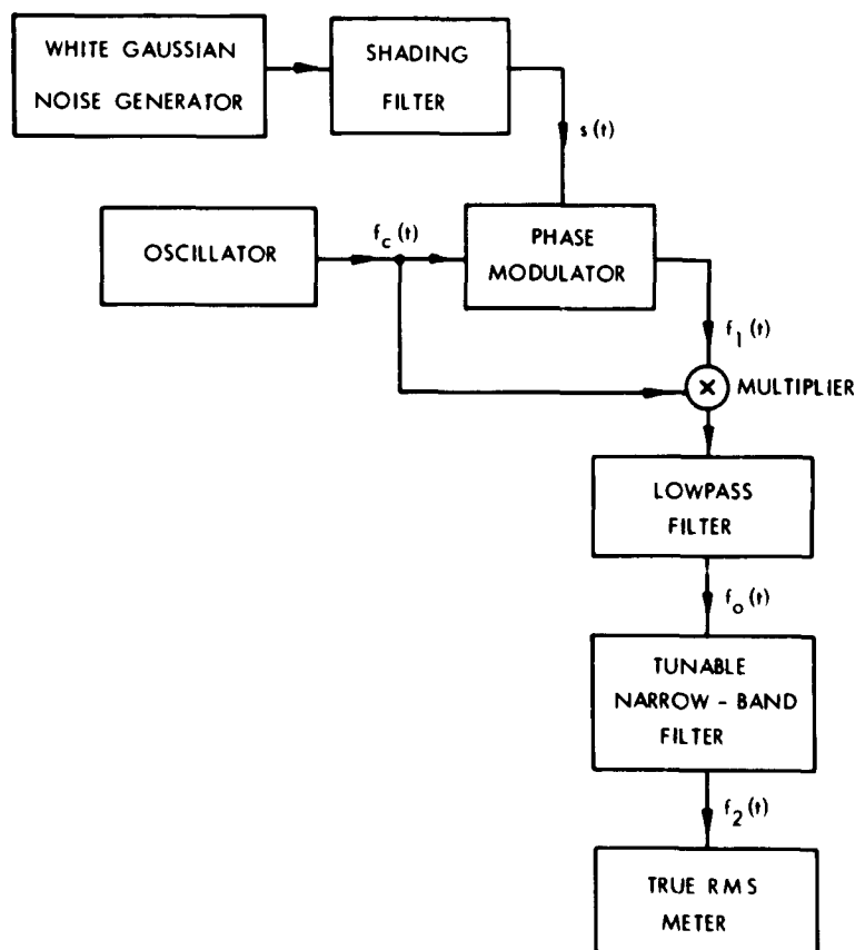
Fig. XIV-21. Experimental system.
