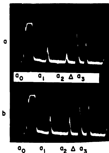
Fig. II-2. (a) Ultrasonic pulses at L-band transmitted through Sample 1 of indium in the normal state. a_0 is rf leakage; a_1 , the first transmitted pulse; a_2 , a superposition of two reflected pulses; \Delta , a calibration pulse; a_3 , a superposition of three reflected pulses (scale, 2 \mu\text{sec/cm} ). (b) Same as in (a) except that the sample is in the superconducting state.
