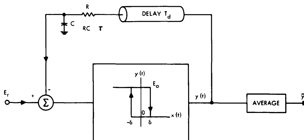
Fig. XIV-4. Regulator. Lower saturation level is set equal to zero to correspond to the voltage regulator example (see Fig. XIV-7).
