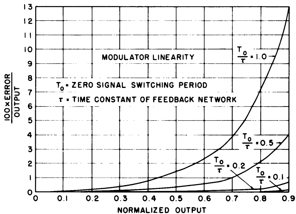
Fig. XIV-2. Modulator nonlinearity vs signal output.
