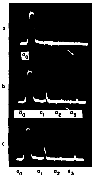
Fig. II-4. (a) Ultrasonic attenuation at L-band in Sample 2 of indium in the normal state. No observable acoustic energy traverses the sample. (b) Same as (a), but in the intermediate state. Note the pulse a_2 , made up of the superposition of the two double reflections. The appearance of this pulse was a random function of the manner in which the magnetic field was changed. (c) Same as (a), but in the superconducting state. Note that a_2 has almost entirely disappeared.
