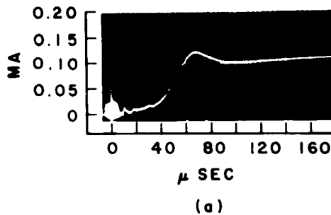
Fig. XII-38. Collected ion currents. V_I = 1000 volts, V_{Acc} = 200 volts, V_N = 100 volts. Transit time, 18 \mu\text{sec} . (a) No electrons: rise time, \sim 60 \mu\text{sec} . (b) With electrons: rise time, \sim 20 \mu\text{sec} .
