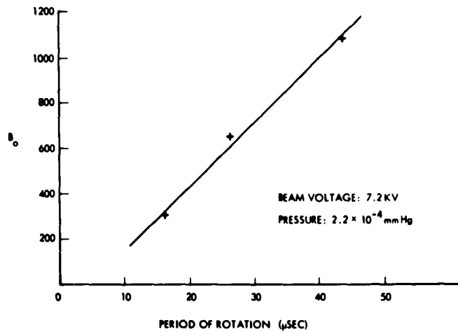
Fig. XII-8. Rotational period vs applied magnetic field.
