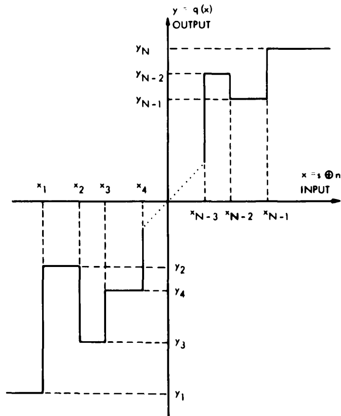
Fig. XIV-10. Input-Output relationship for a quantizer.
