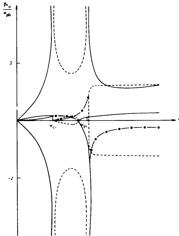
Figure XII-20. Dispersion for \frac{n_b}{n_p} \frac{T_e}{2V_o} = 1 .
