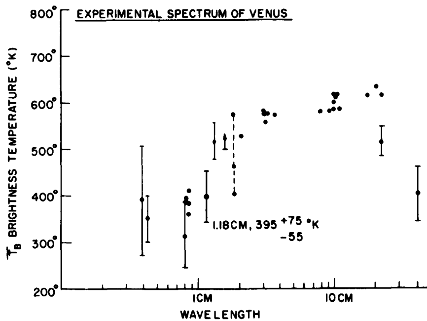
Fig. VII-2. Radiofrequency spectrum of Venus.
