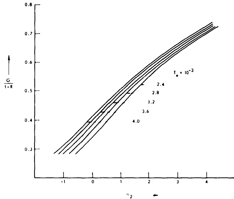
Fig. XIII-6. \frac{G}{1-R}(\eta_2) for T_E = 1600^\circ\text{K} , T_e = 1200^\circ\text{K} .
