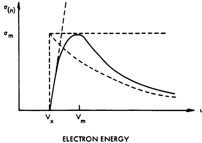
Fig. XI-1. Approximate excitation and ionization cross sections.
