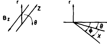
Fig. XII-24. Coordinate system for derivation of the orbital equations.
