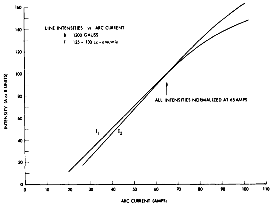
Fig. XI-4. Line intensities vs arc current.
