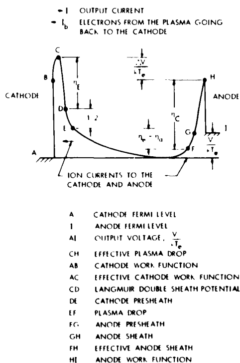
Fig. XIII-4. Motive diagram for the Langmuir mode.
