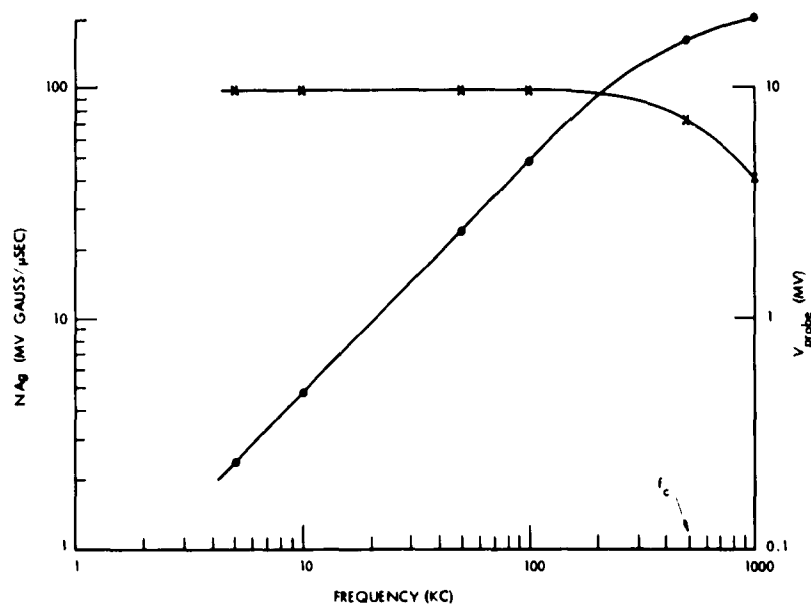
Fig. XII-2. Plot of V_{\text{probe}} vs frequency (...) and plot of N\Delta g vs frequency (xxx) at constant current, 0.01 amp (1 amp = 7.8 gauss).
