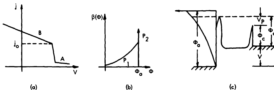
Fig. XIII-10. (a) Typical I-V curve; (b) Distribution of work function; (c) Motive diagram for operation in region B.
