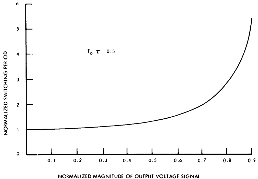
Fig. XIV-3. Switching period vs magnitude of output signal.
