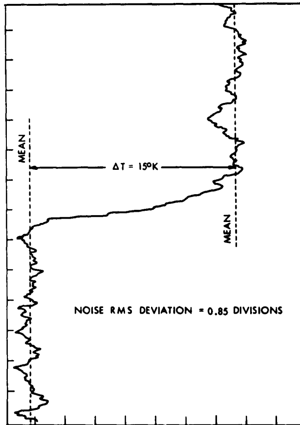
Fig. VII-6. Radiometer output with 4-sec integration time.
