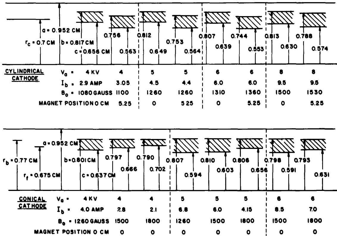
Fig. V-4. Beam dimensions.
