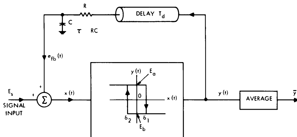
Fig. XIV-1. Modulation system with system parameters indicated.
