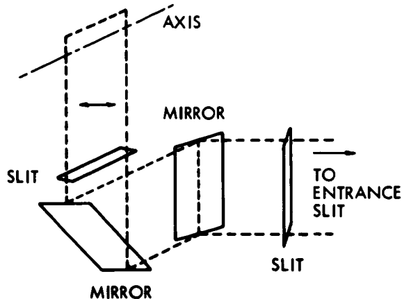
Fig. XI-3. Movable collimator.
