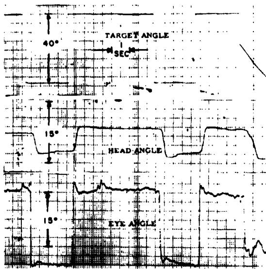
Fig. XXII-10. Typical responses to square step input.
