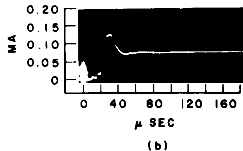
Fig. XII-38. Collected ion currents. V_I = 1000 volts, V_{Acc} = 200 volts, V_N = 100 volts. Transit time, 18 \mu\text{sec} . (a) No electrons: rise time, \sim 60 \mu\text{sec} . (b) With electrons: rise time, \sim 20 \mu\text{sec} .
