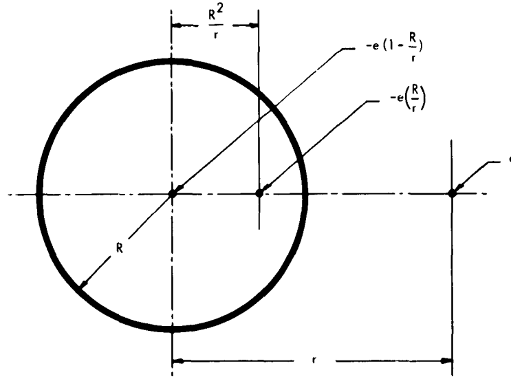
Fig. XIII-13. Induced charges in the spherical conductor.
