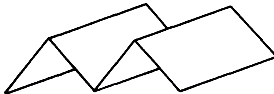
Fig. XX-6. The illusion.
