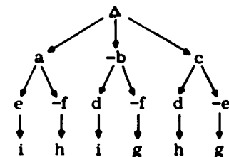
The Determinant Tree
