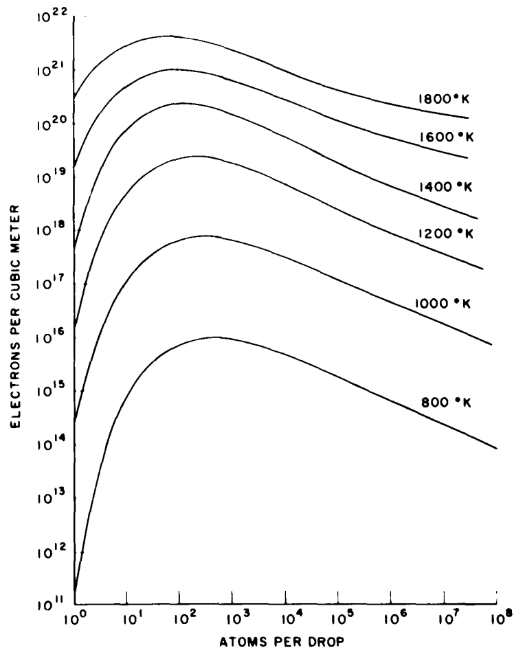
Fig. XIII-14. Electron density in wet potassium vapor.
