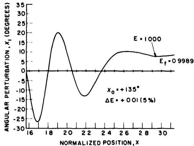
Fig. XII-29. Angular deviation versus x for the corkscrew of Fig. XII-28. In this case, the initial perturbation was in energy.
