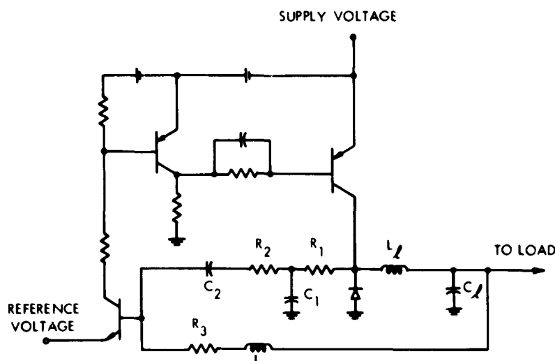
Fig. XIV-7. Voltage regulator that exemplifies nonlinear control.
