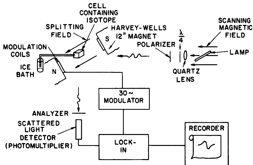
Fig. IV-1. Experimental arrangement for level-crossing work.
