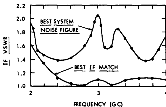
Fig. VII-3. VSWR at I-F port versus frequency.
