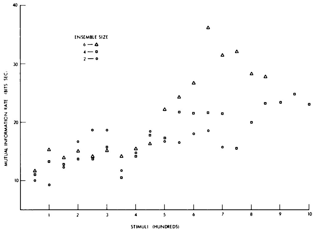
Fig. XXIII-5. Learning curves.
