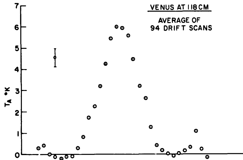
Fig. VII-1. Average of 94 drift scans of Venus.
