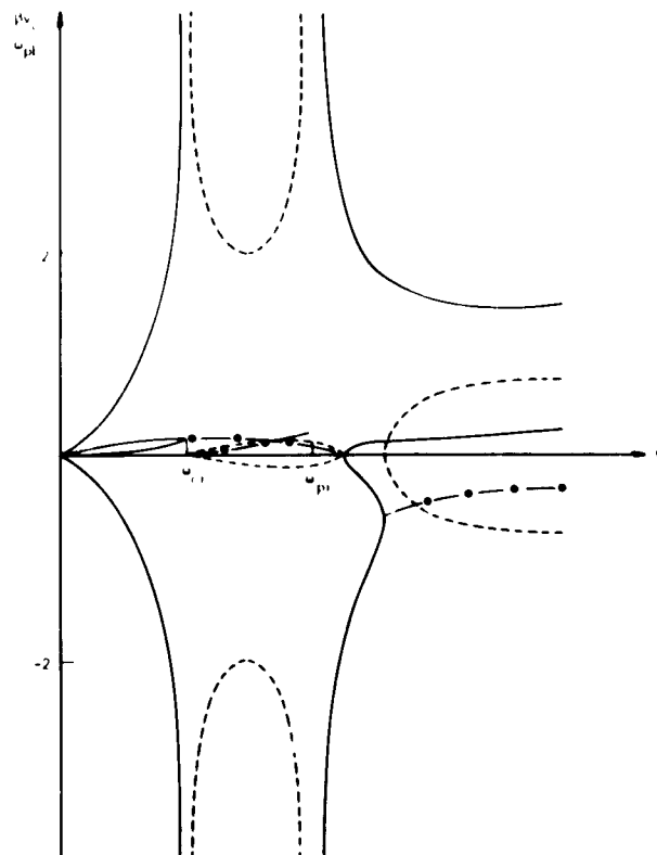
Figure XII-21. Dispersion for T_e = \infty .
