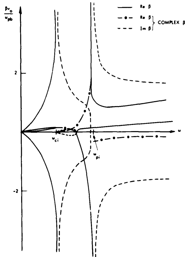
Fig. XII-19. Dispersion for \frac{n_b}{n_p} \frac{T_e}{2V_o} = 0.5 .
