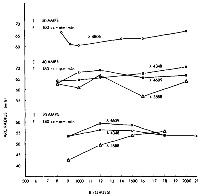
Fig. XI-6. Arc width vs magnetic field.
