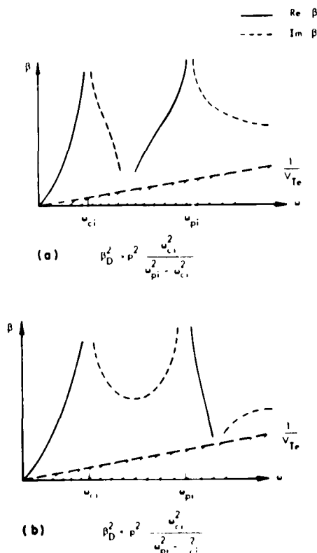
Fig. XII-18. Dispersion in a hot electron plasma.
