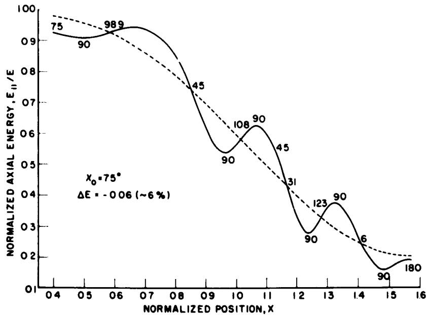
Fig. XII-27. Normalized z-directed energy versus x . The conditions for this case differ from those of Fig. XII-26 only in the value of x_0 . x is the running parameter.
