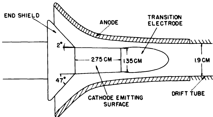
Fig. V-9. Conical-cathode magnetron injection gun.
