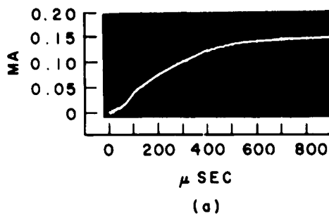
Fig. XII-37. Collected ion currents. V_I = 600 volts, V_{Acc} = 100 volts, V_N = 0 . Transit time, 22 \mu\text{sec} . (a) No electrons: rise time, \sim 500 \mu\text{sec} . (b) With electrons: rise time, \sim 25 \mu\text{sec} .
