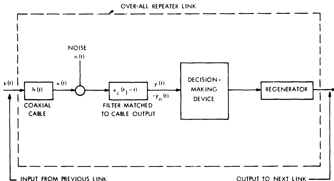
Fig. XIV-11. Block diagram of the system.
