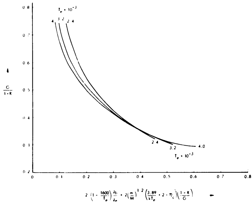
Fig. XIII-8. Back emission and ionization losses. T_E = 1600^\circ K , T_p = 1200^\circ K .
