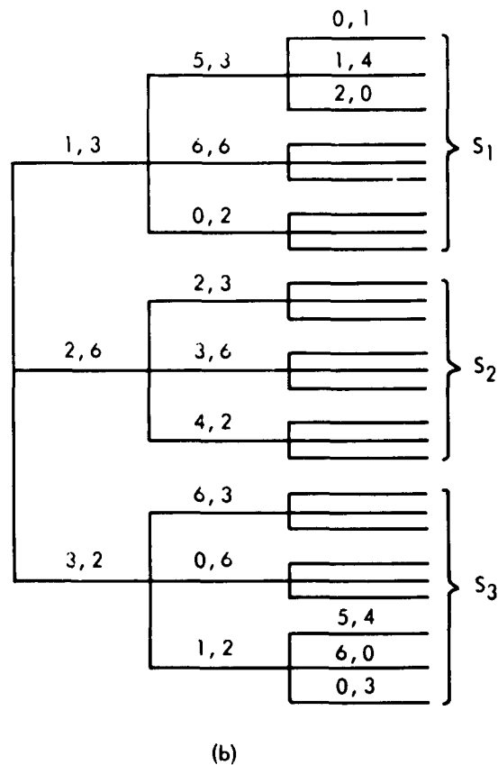
Fig. XV-3. (a) Generator function g(t) . (b) Tree code generated by g(t) and the set of field elements 1, 2, 3.
