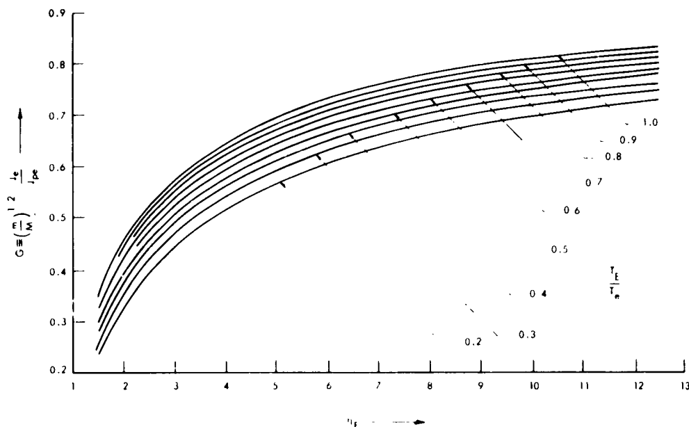
Fig. XIII-5. Langmuir double-sheath condition T_p \text{ eff} = 0.5T_e .
