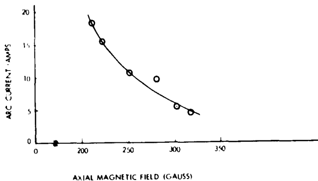
Fig. XII-14. Minimum axial magnetic field for instability vs arc current.
