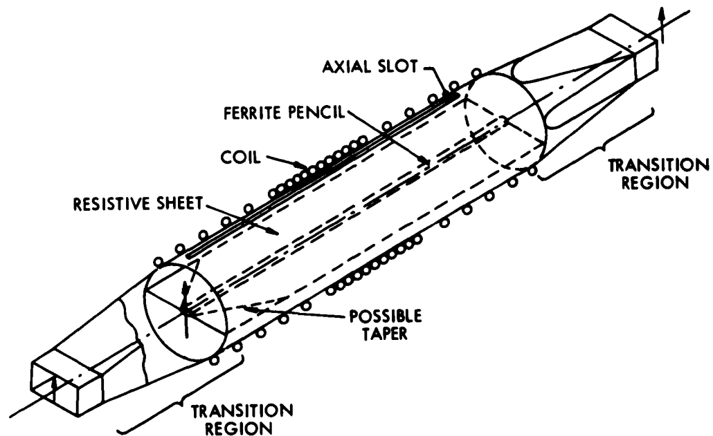
Fig. VII-7. Broadband ferrite switch.
