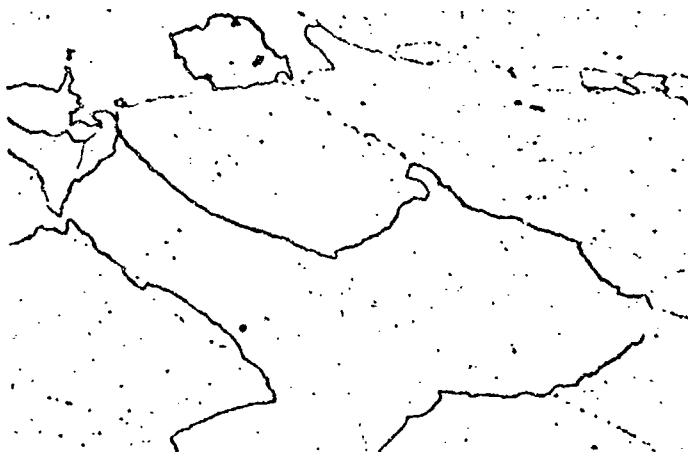
Solution Treated Condition, 285 BHN Microstructure consists essentially of single phase matrix. Magnification: 100X Etchant: 1 part HF 1 part HNO 3 2 parts Glycerol
