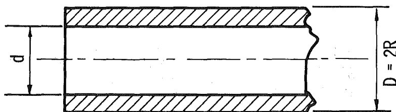
Flat-Nosed Probe
