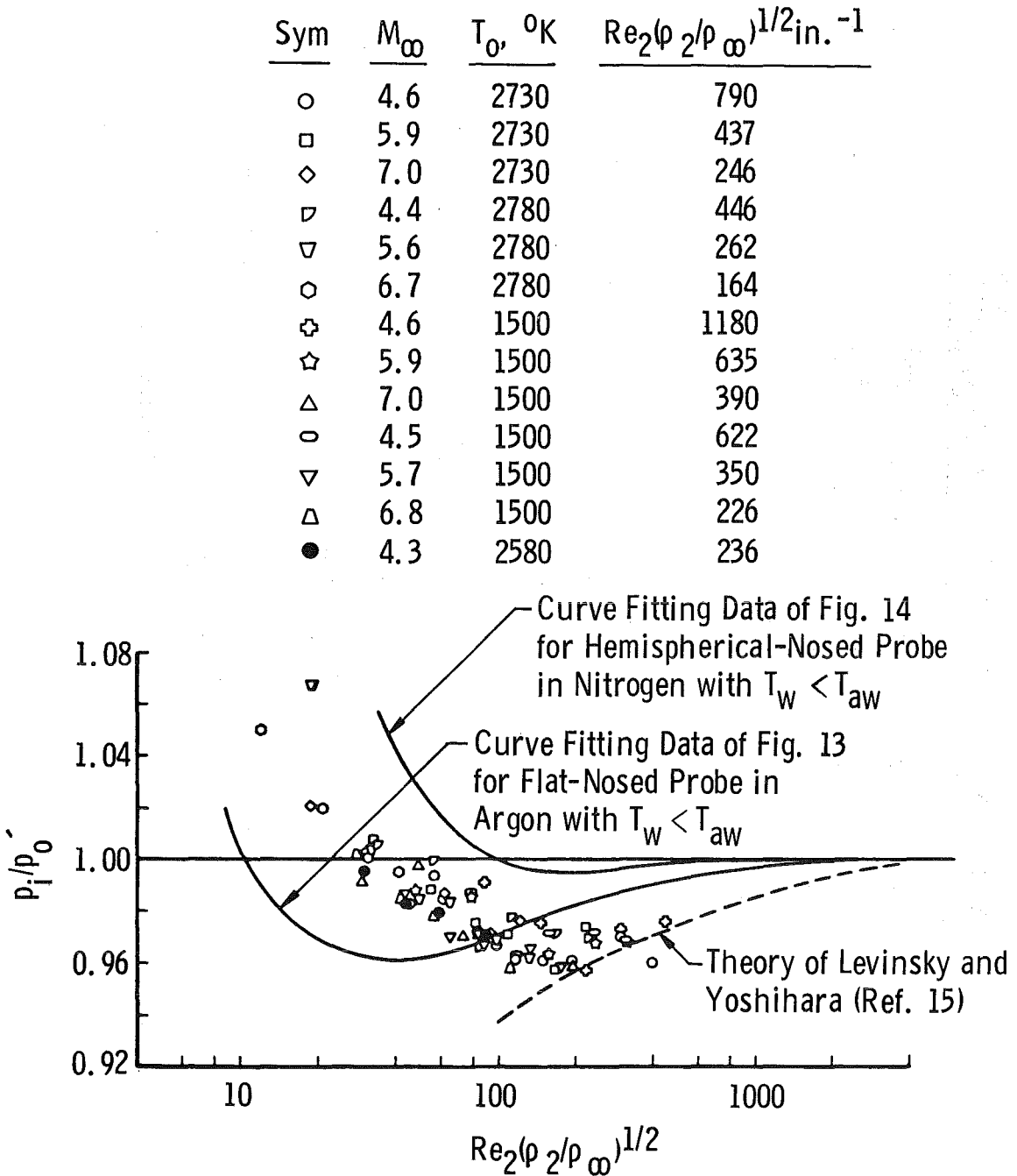
Fig. 15 AEDC-VKF Data for Hemispherical-Nosed Probes in Argon with T_w = 0.1 to 0.2 T_0 .
