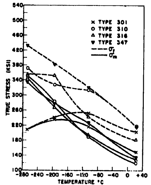
Figure 9. 300 Series Stainless Steels EFFECT OF TEMPERATURE ON TRUE STRESS AT FRACTURE AND MAXIMUM LOAD
