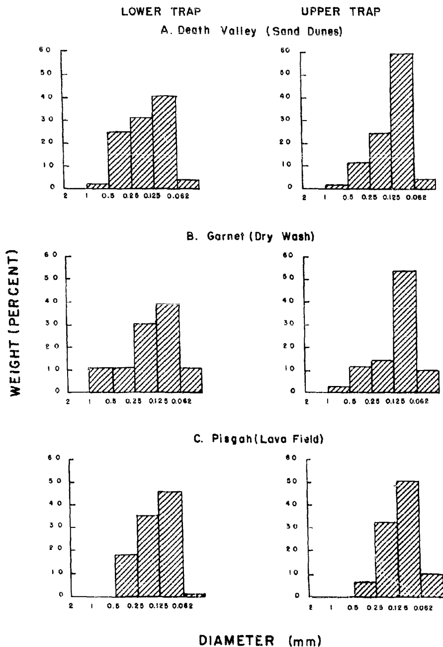
Figure 32. Histograms showing grain size variation with increasing height above the surface.
