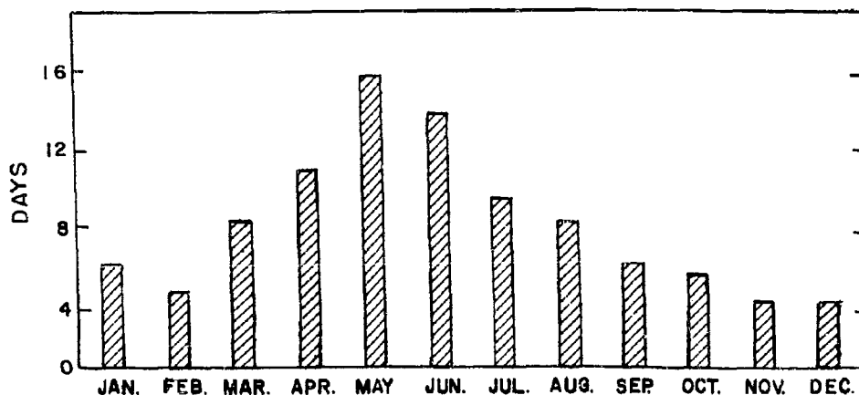
Figure 5. Days per month with winds over 20 mph at Thermal Airport in Coachella Valley, California.
