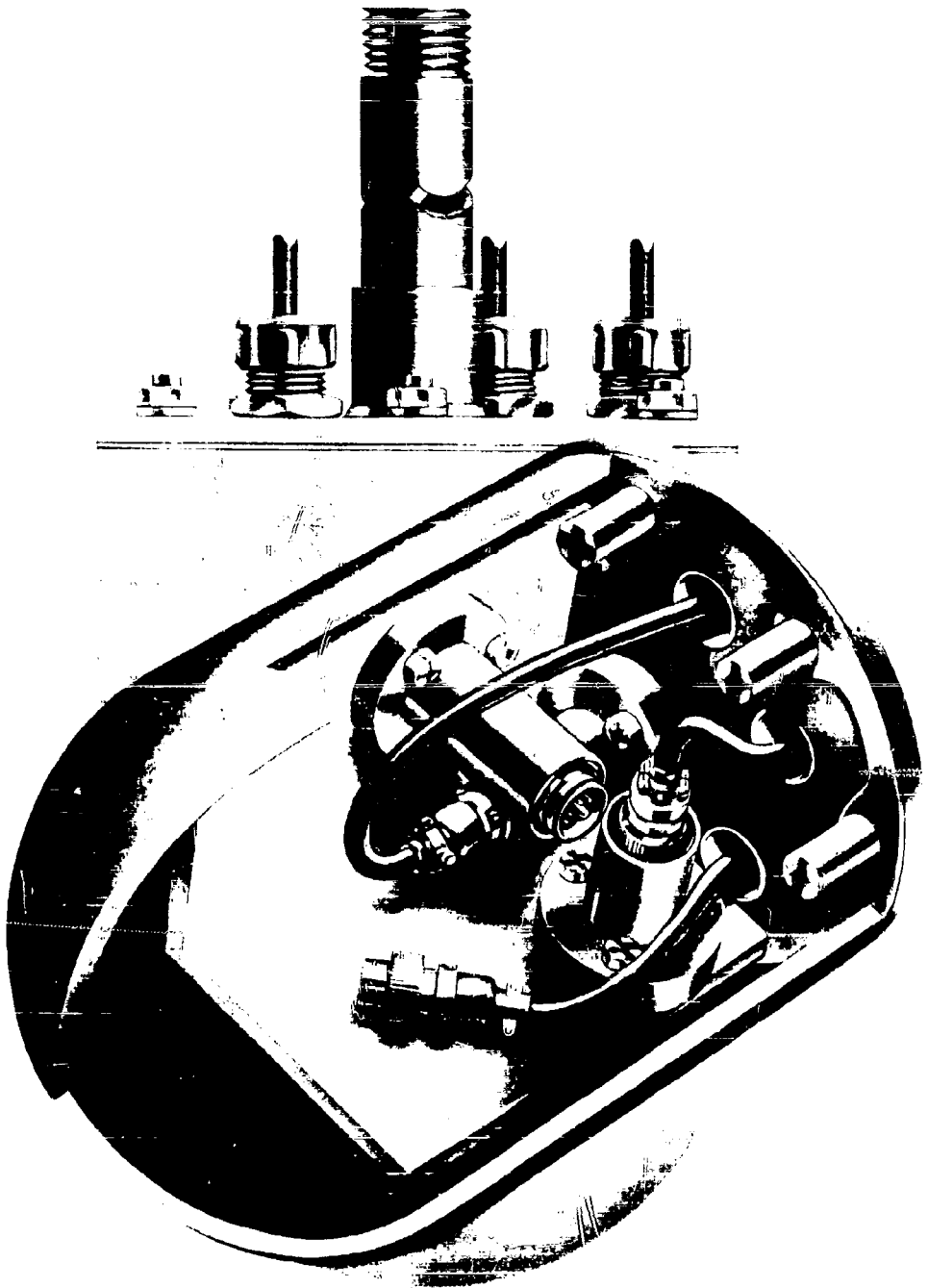
Fig. 2.4 Three-Component Accelerometer Mount
