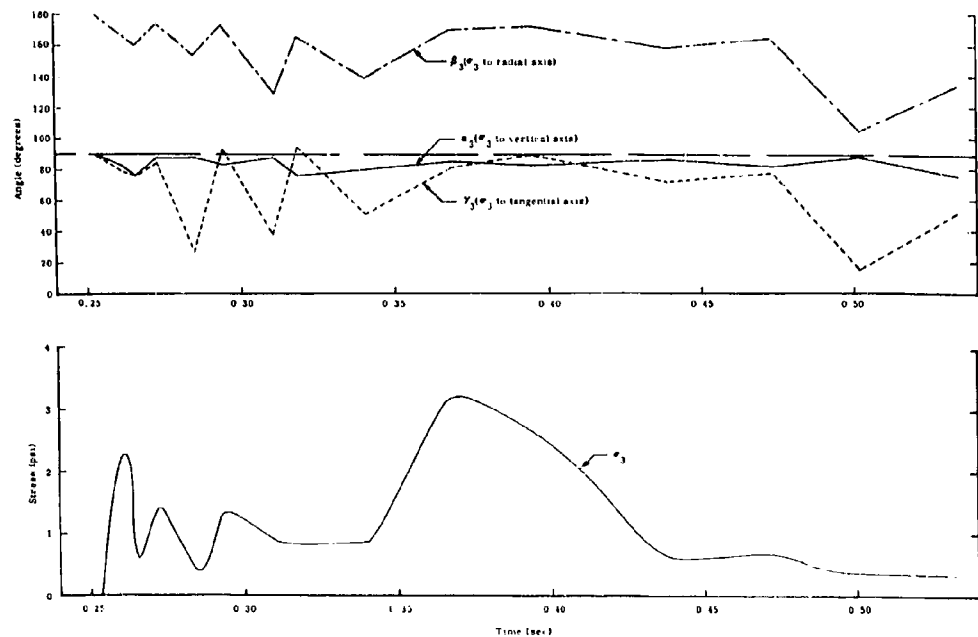
Fig. 2.15 Minor Principal Stress and Orientation vs Time - Shot 10
