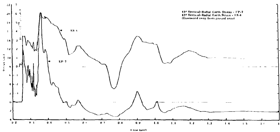
Fig. C.18 Earth Stress and Strain vs Time - Shot 10
