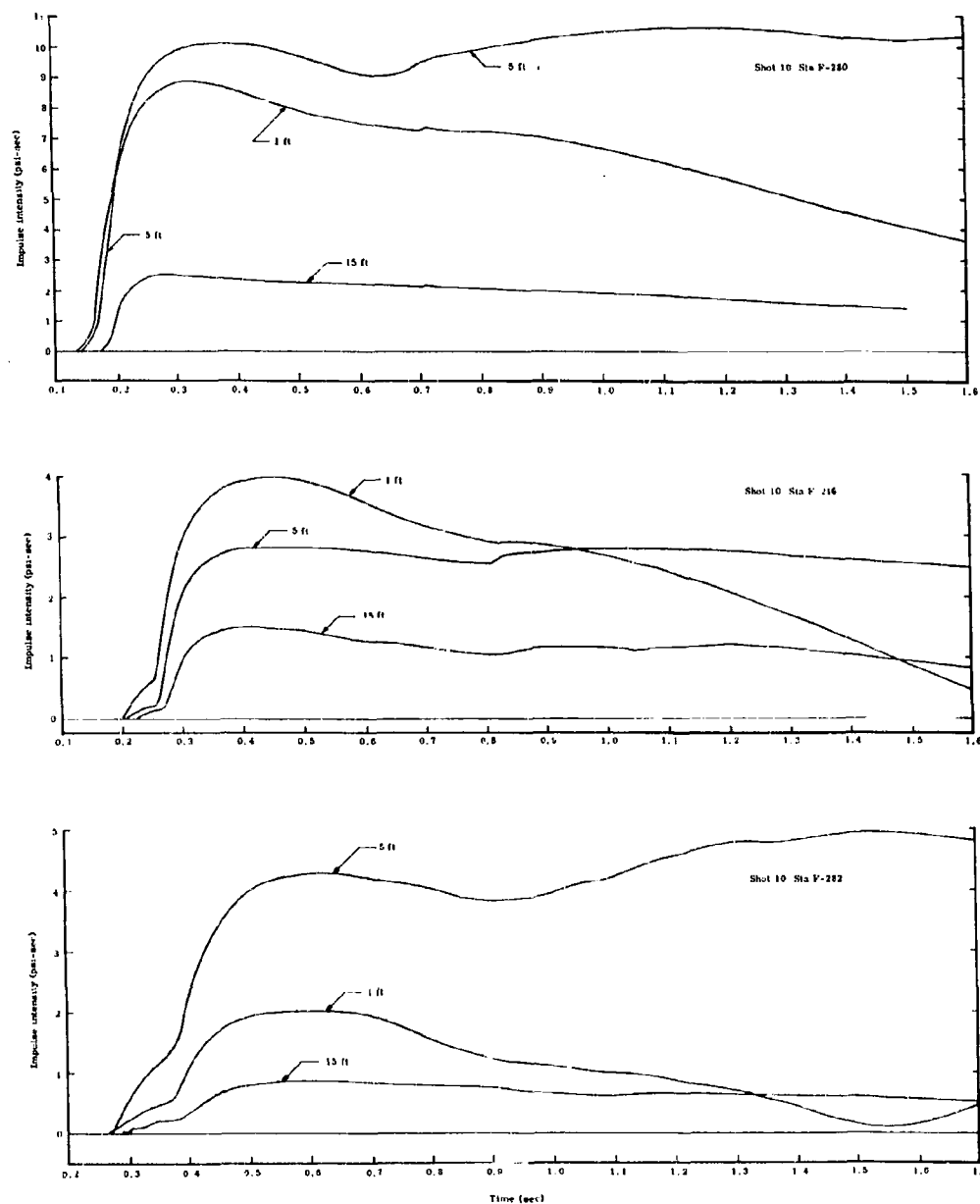
Fig. A.8 Impulse Intensity vs Time vs Depth
