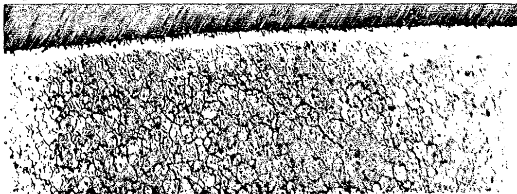
Film and Slight Intergranular Oxidation
