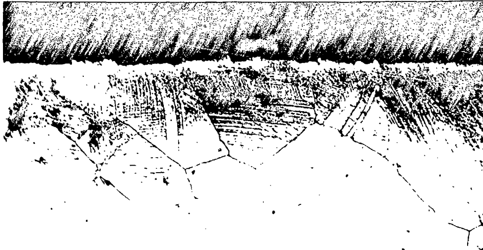
Scale Oxidation
