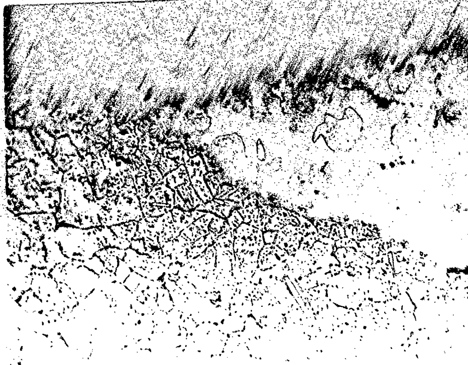
Extreme Pitting and Corrosive Alloying
