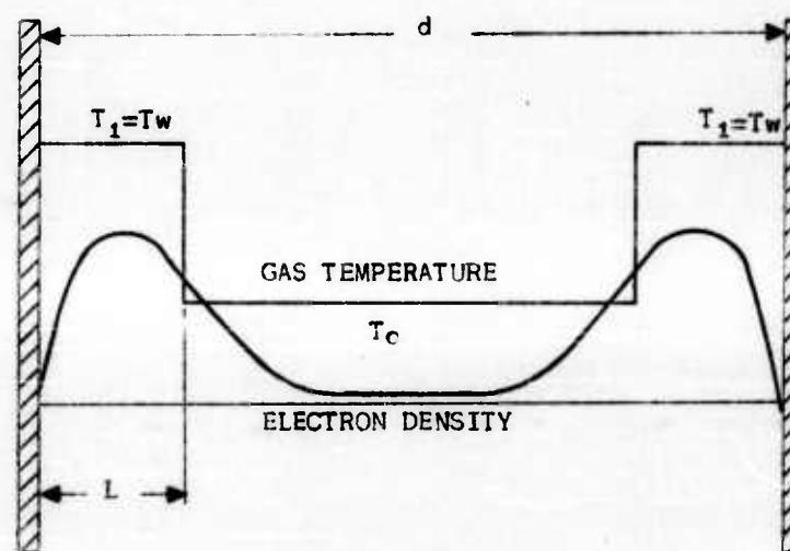
FIGURE 6 PHYSICAL MODELS USED IN ANALYZING BREAKDOWN AT HOT SURFACES
