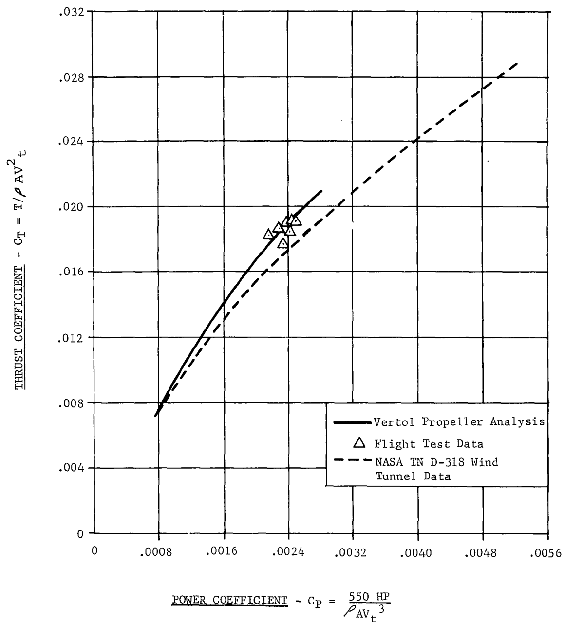
FIGURE 29. THRUST COEFFICIENT VS POWER COEFFICIENT (HOVER CONFIGURATION)
