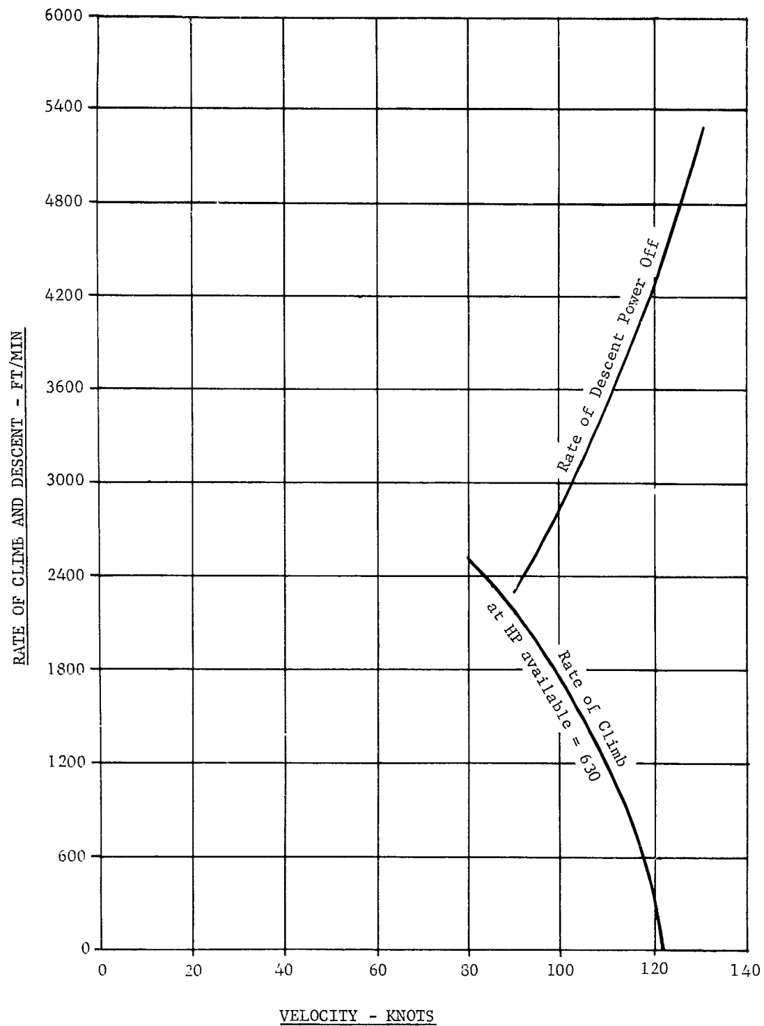
FIGURE 30. RATE OF CLIMB AND DESCENT VS VELOCITY (AIRPLANE CONFIGURATION)
