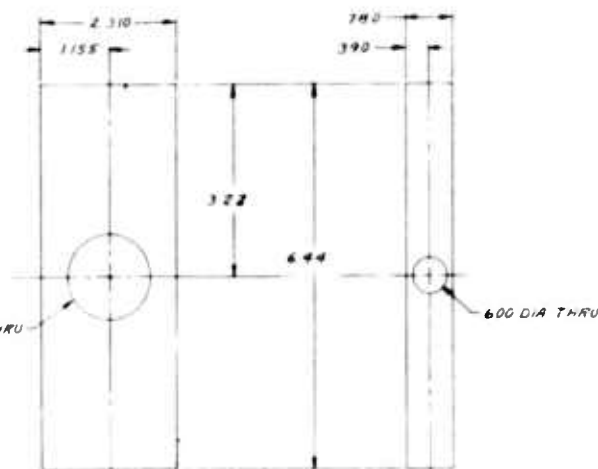
DETAIL OF DASH 20 2 PLACES STOCK THICKNESS: .060
