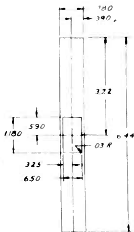
DETAIL OF DASH 19 STOCK THICKNESS: .060
