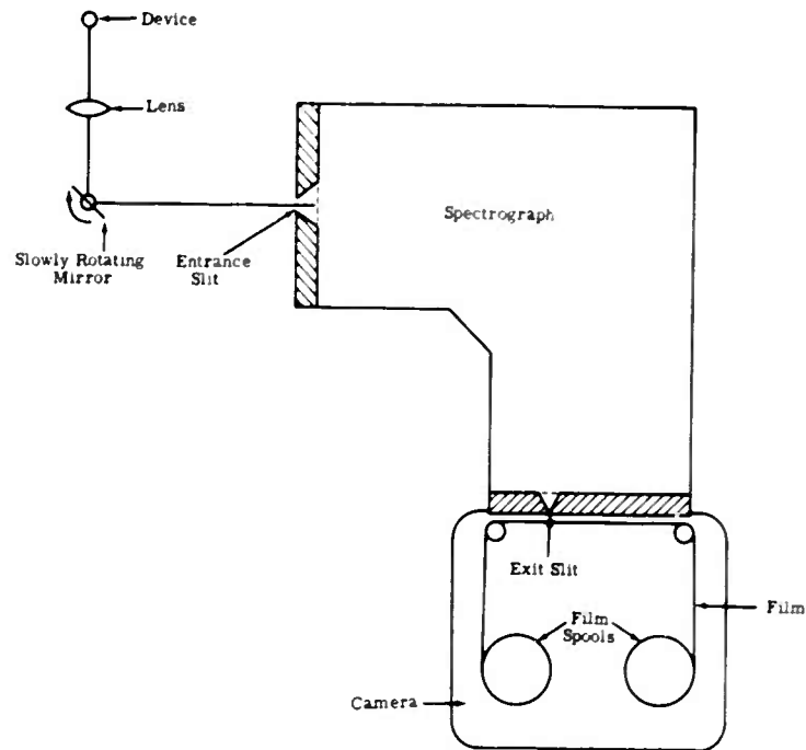
Figure 20. Schematic Diagram of Optical Arrangement
