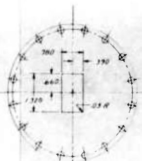
DETAIL OF DASH 15 SAME AS DASH 17 EXCEPT AS SHOWN
