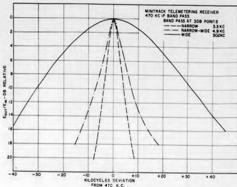
Fig. 4 - Minitrack telemetering receiver 470-kc i-f bandpass
