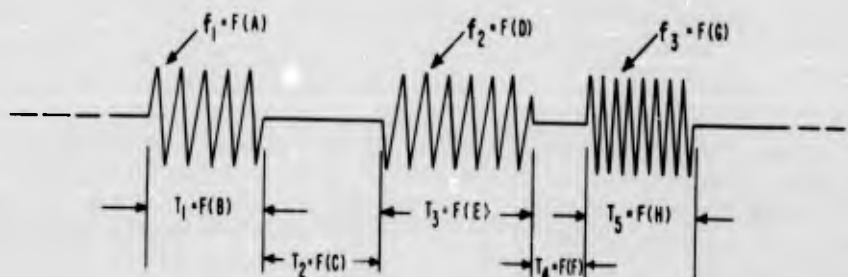
Fig. 1 - Telemetry modulation waveform
