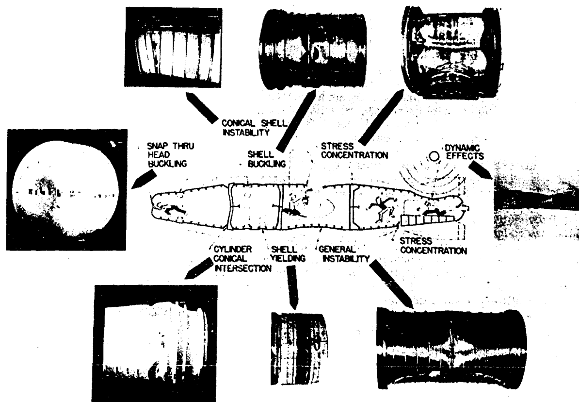
Fig. 8 - Possible modes metal of failure due to hydrostatic pressure
