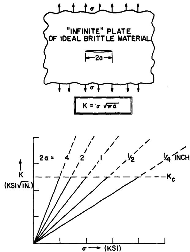
Fig. 2 - Stress intensity parameter, K , as a function of nominal stress normal to the crack and of crack length for a thin, "infinite" plate of an ideally brittle material
