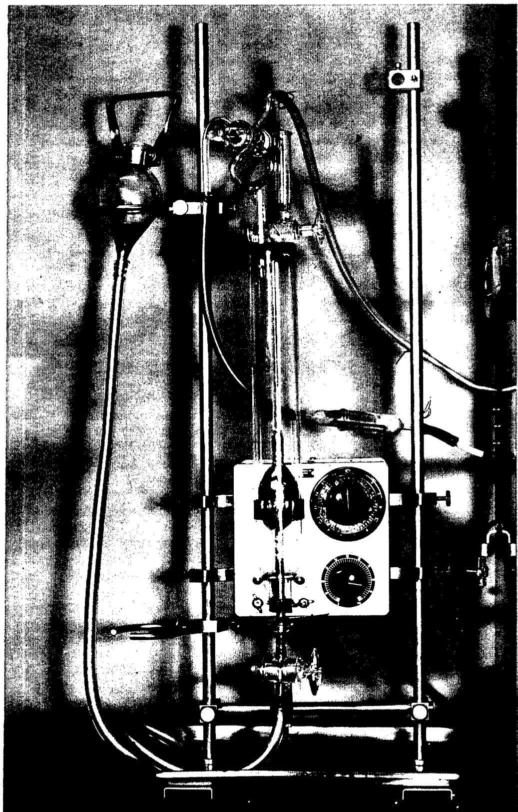
Figure 2. Van Slyke apparatus for liberating carbon monoxide from biologic specimens, modified for introducing released gas into the gas chromatograph.
